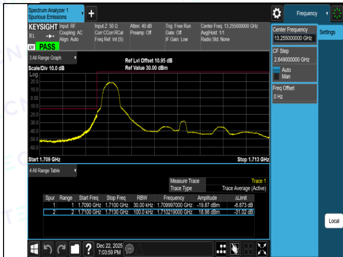
Band66-3MHz-QPSK-131987-15RB#0-PASS
