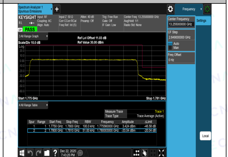
Band66-5MHz-16QAM-131997-1RB#24-PASS
