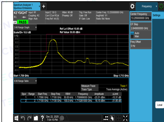
Band66-3MHz-16QAM-131987-15RB#0-PASS
