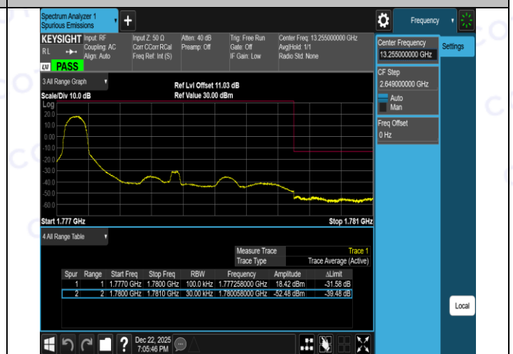
Band66-3MHz-16QAM-132657-15RB#0-PASS
