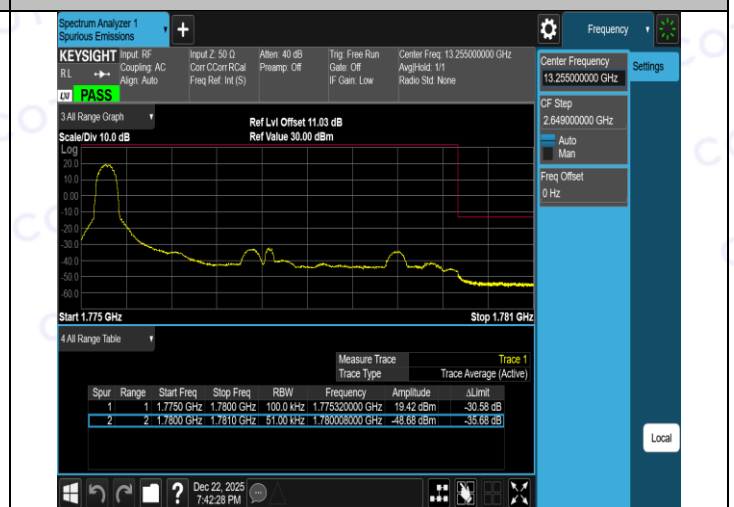
Band66-5MHz-QPSK-132647-25RB#0-PASS
