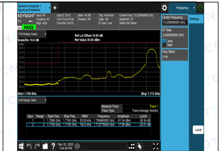
Band66-3MHz-16QAM-132657-1RB#0-PASS
