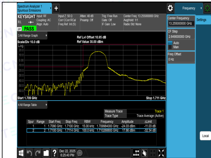
Band66-1.4MHz-16QAM-131979-6RB#0-PASS
