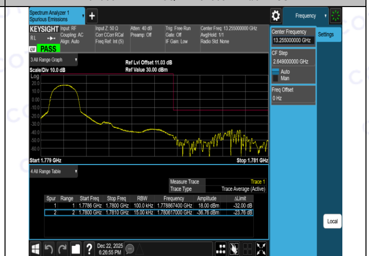
Band66-1.4MHz-16QAM-132665-6RB#0-PASS
