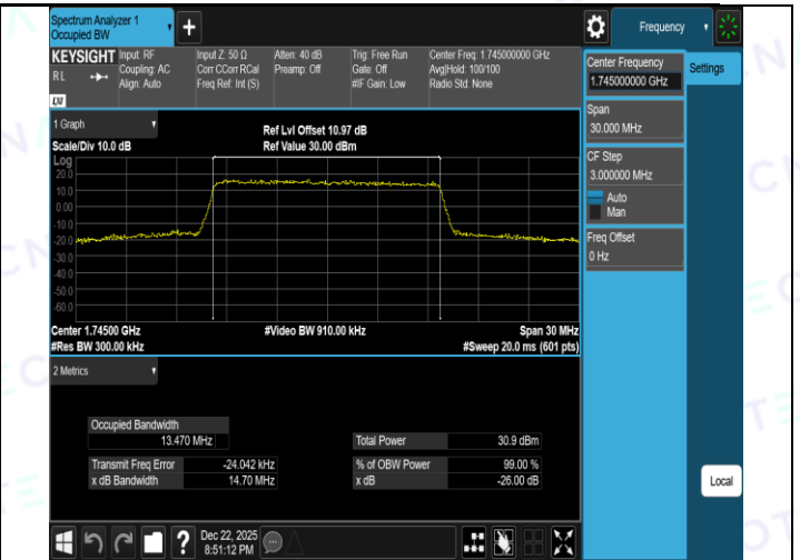
Band66-15MHz-16QAM-132047-75RB#0-PASS
