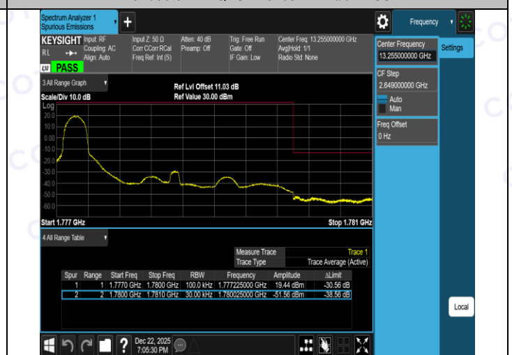
Band66-3MHz-QPSK-132657-15RB#0-PASS
