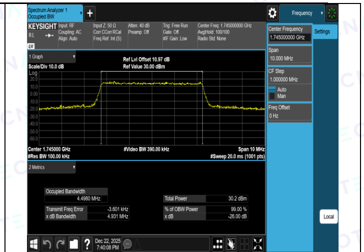
Band66-5MHz-16QAM-131997-25RB#0-PASS
