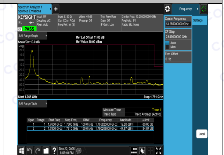
Band66-15MHz-QPSK-132597-75RB#0-PASS
