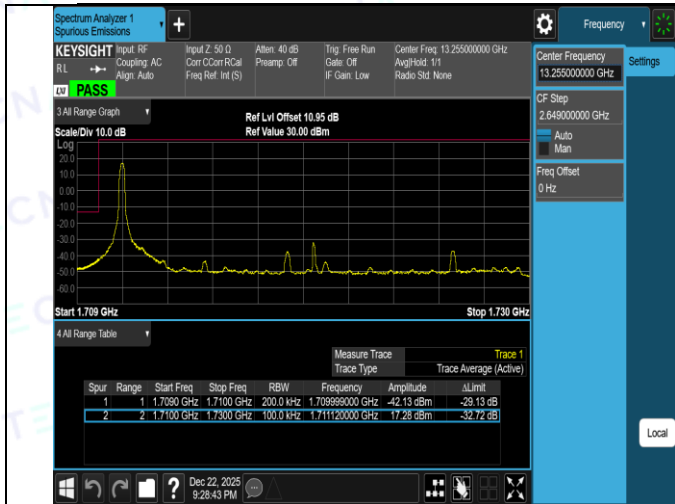
Band66-20MHz-16QAM-132072-100RB#0-PASS
