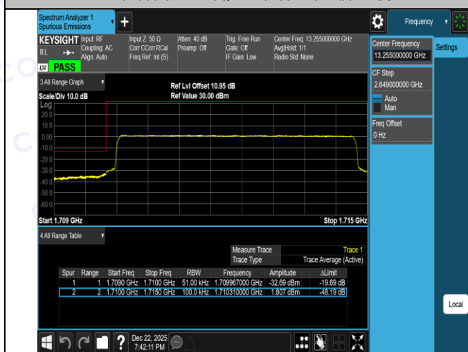
Band66-5MHz-16QAM-132647-1RB#24-PASS
