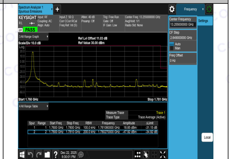
Band66-20MHz-QPSK-132572-100RB#0-PASS
