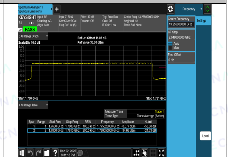
Band66-20MHz-16QAM-132572-100RB#0-PASS
