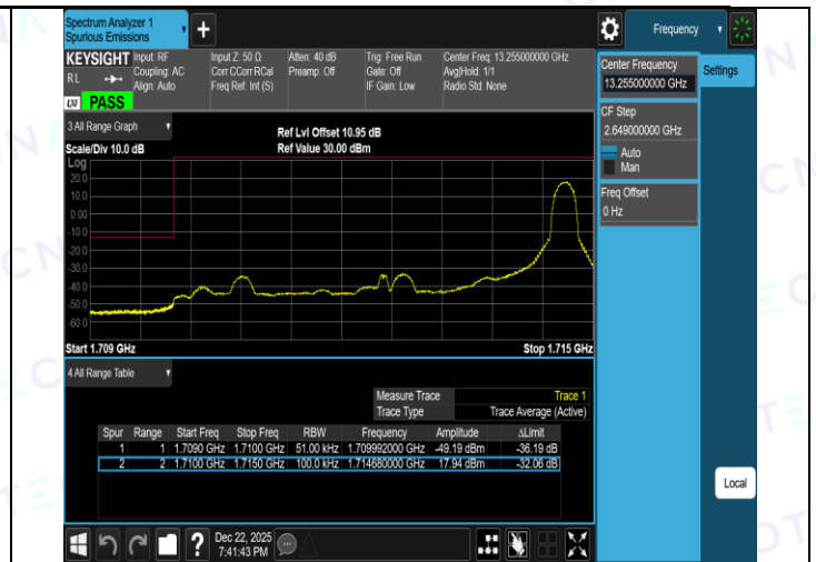
Band66-5MHz-16QAM-132647-1RB#0-PASS
