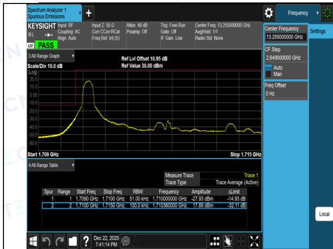
Band66-5MHz-16QAM-131997-25RB#0-PASS
