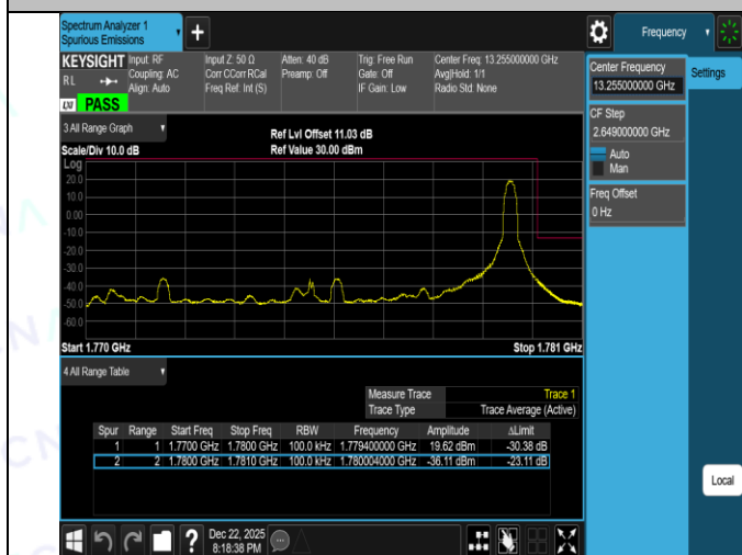
Band66-10MHz-16QAM-132022-1RB#0-PASS
