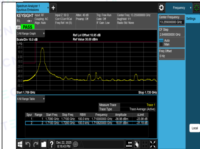
Band66-10MHz-QPSK-132022-50RB#0-PASS
