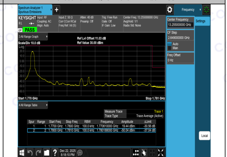
Band66-10MHz-QPSK-132622-50RB#0-PASS
