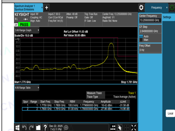
Band66-10MHz-QPSK-132022-1RB#0-PASS
