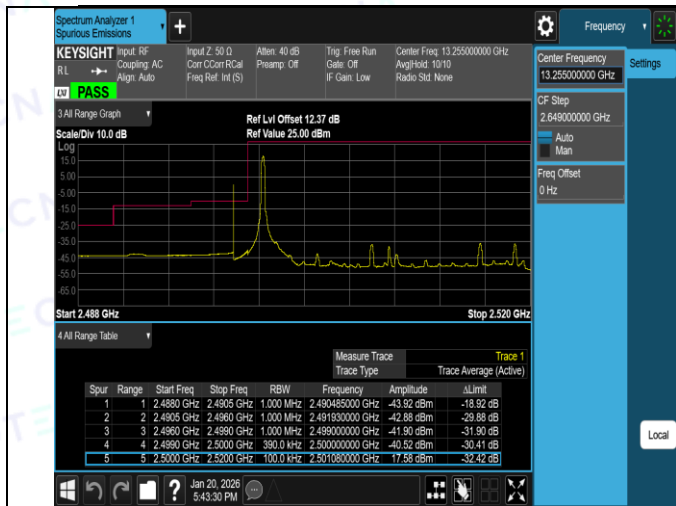
Band7-20MHz-QPSK-20850-100RB#0-PASS
