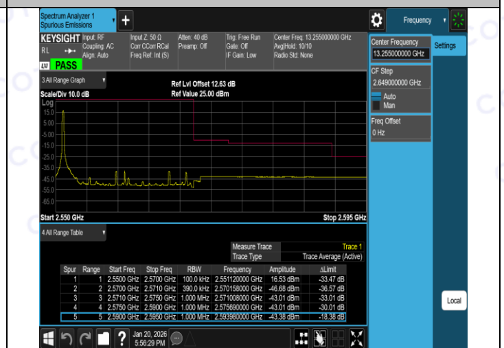
Band7-20MHz-16QAM-21350-100RB#0-PASS
