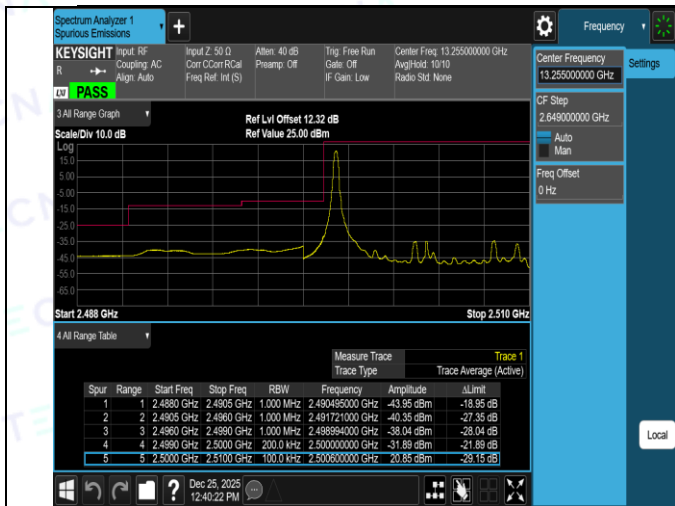
Band7-10MHz-16QAM-20800-50RB#0-PASS
