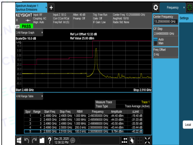
Band7-10MHz-QPSK-20800-50RB#0-PASS
