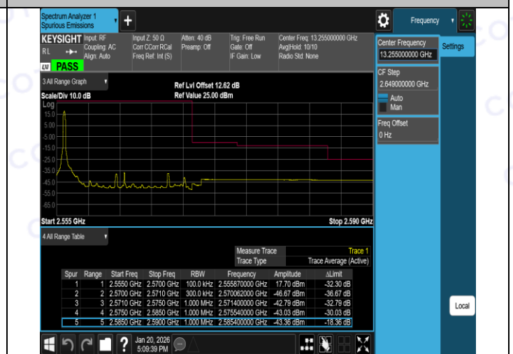
Band7-15MHz-QPSK-21375-75RB#0-PASS
