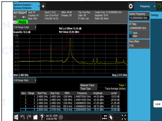
Band7-15MHz-16QAM-20825-75RB#0-PASS
