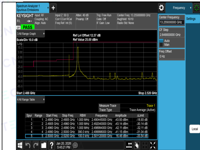
Band7-20MHz-16QAM-20850-100RB#0-PASS
