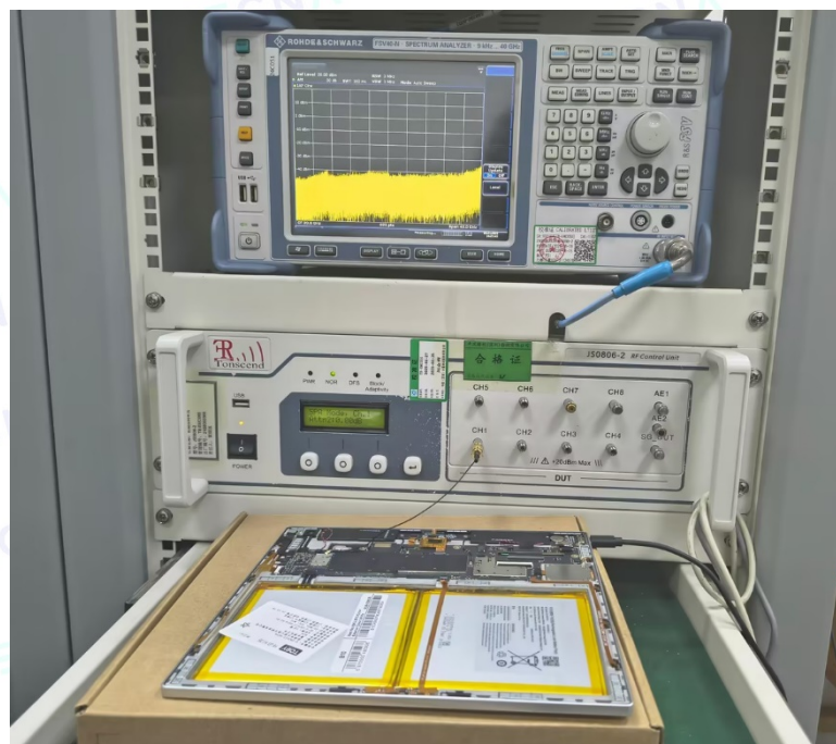
Conducted Measurements Test (WIFI)
