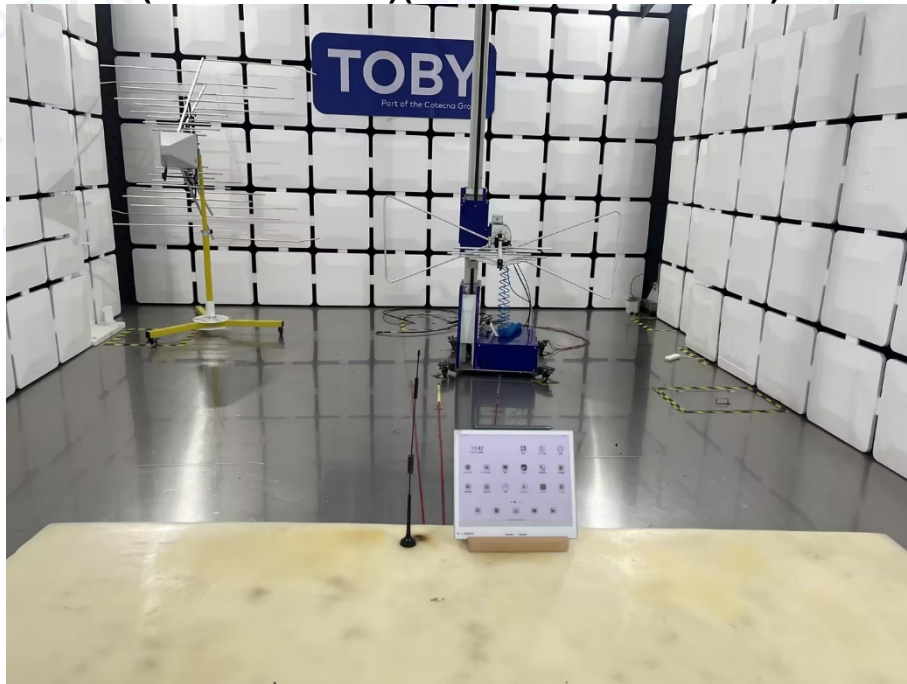
Photo of Setup for Radiated Emission (30MHz~1GHz)(GSM&WCDMA&LTE)
