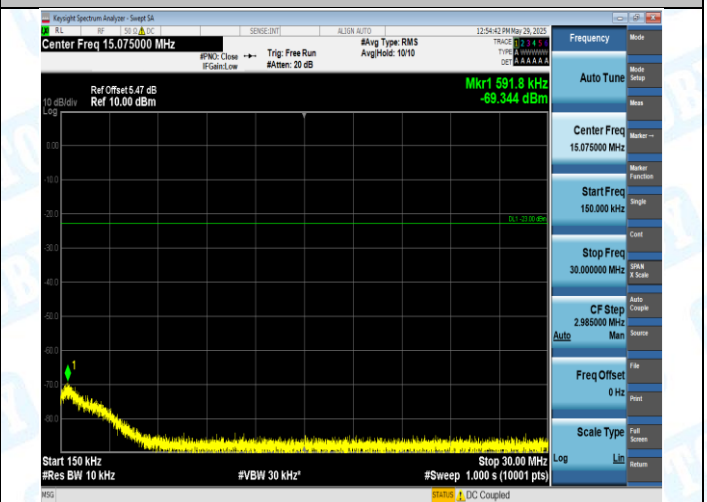
EGPRS850-190-8-0.15~30MHz-PASS
