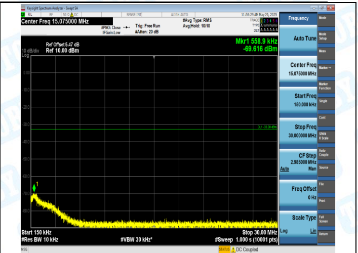
EGPRS1900-512-2-0.15-30MHz-PASS
