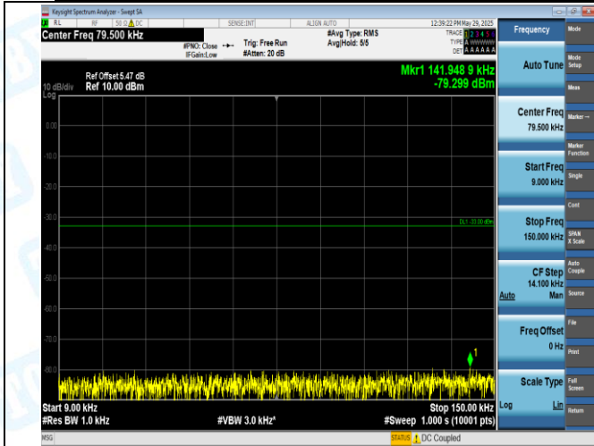
EGPRS850-128-8-0.009~0.15MHz-PASS
