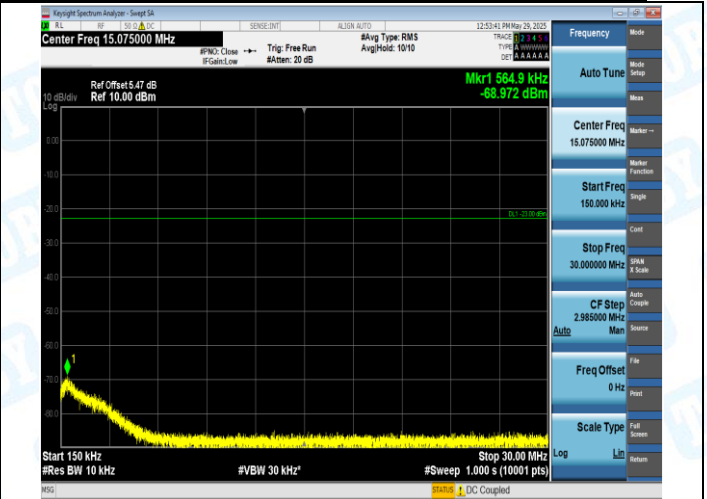
EGPRS850-128-8-0.15~30MHz-PASS
