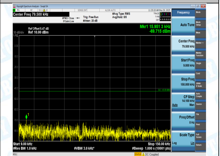
EGPRS1900-661-2-0.009-0.15MHz-PASS
