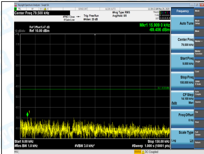
EGPRS1900-512-2-0.009-0.15MHz-PASS
