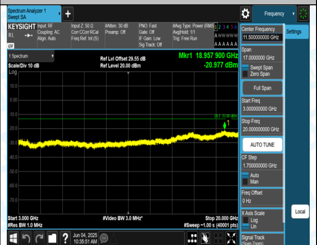
Band2-3MHz-QPSK-18900-1RB#0-3000~20000-PASS
