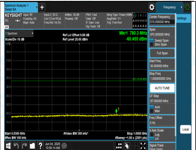
Band2-1.4MHz-QPSK-18900-1RB#0-30-1000-PASS
