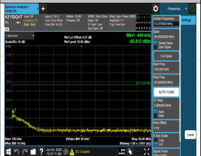
Band2-3MHz-QPSK-19185-1RB#0-0.15~30-PASS
