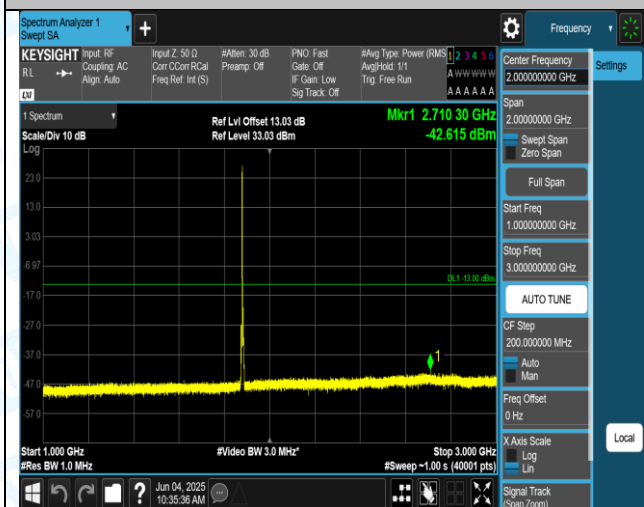
Band2-3MHz-QPSK-18900-1RB#0-1000~3000-PASS
