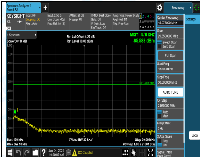
Band2-1.4MHz-QPSK-18900-1RB#0-0.15-30-PASS
