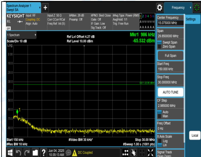
Band2-3MHz-QPSK-18900-1RB#0-0.15~30-PASS
