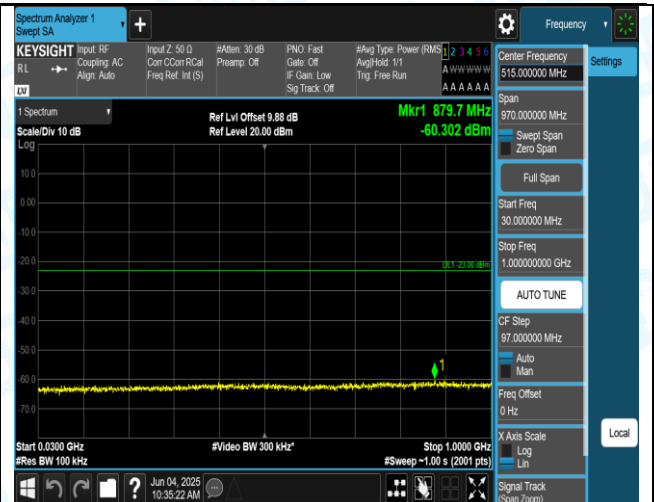
Band2-3MHz-QPSK-18900-1RB#0-30~1000-PASS
