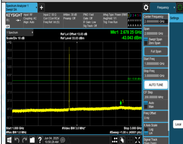
Band2-1.4MHz-QPSK-18900-1RB#0-1000-3000-PASS
