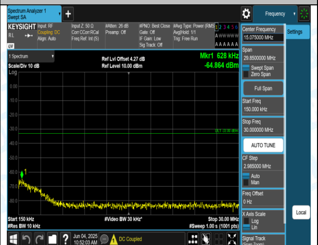
Band2-1.4MHz-QPSK-19193-1RB#0-0.15-30-PASS
