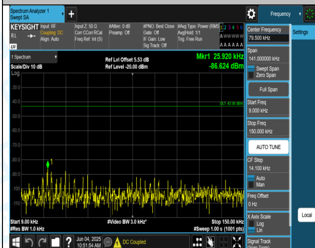
Band2-1.4MHz-QPSK-19193-1RB#0-0.009-0.15-PASS
