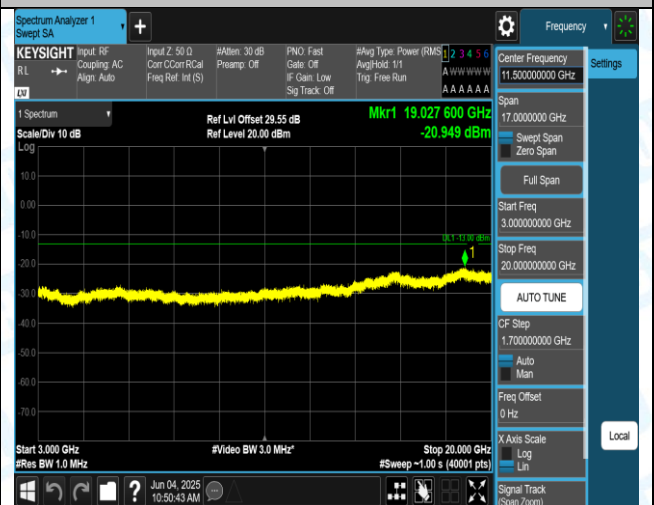
Band2-1.4MHz-QPSK-18900-1RB#0-3000-20000-PASS
