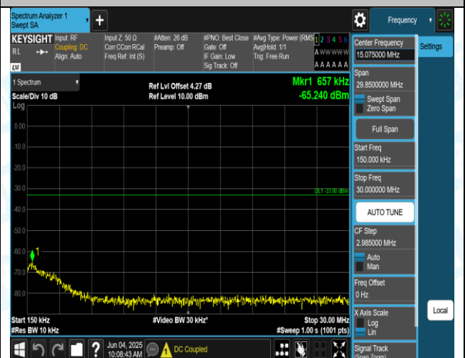
Band2-10MHz-QPSK-19150-1RB#0-0.15-30-PASS
