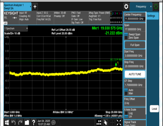
Band2-10MHz-QPSK-18900-1RB#0-3000-20000-PASS
