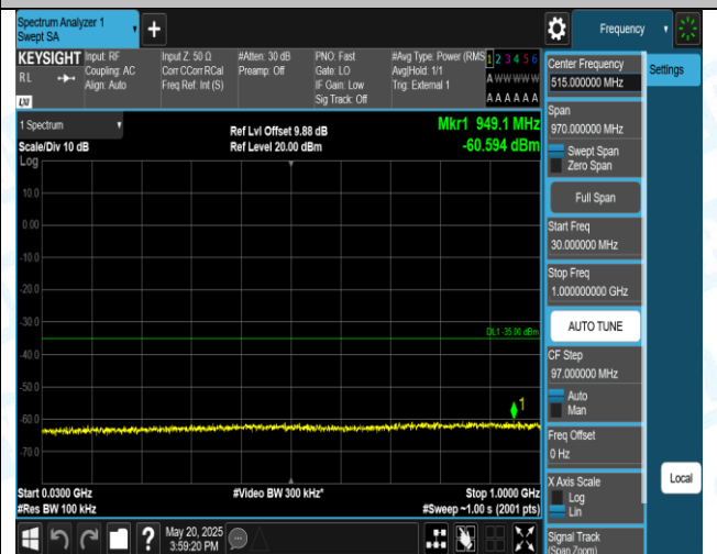
Band38-10MHz-16QAM-37800-1RB#0-30~1000-PASS
