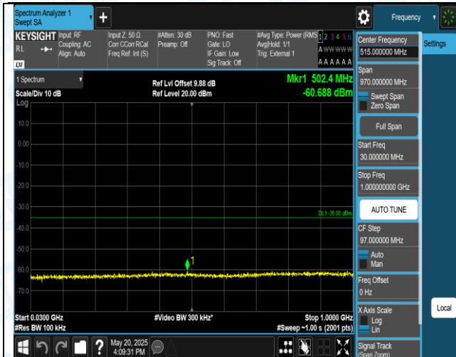
Band38-10MHz-QPSK-38200-1RB#0-30~1000-PASS
