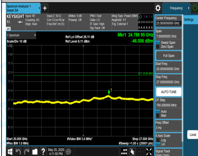
Band38-10MHz-QPSK-38200-1RB#0-20000~27000-PASS
