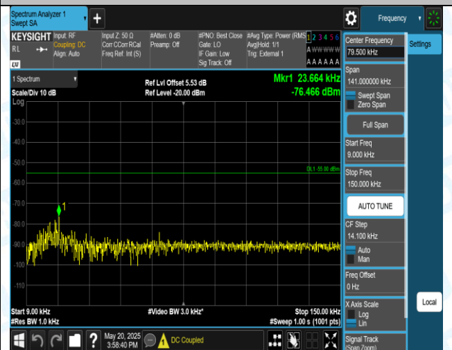
Band38-10MHz-16QAM-37800-1RB#0-0.009~0.15-PASS
