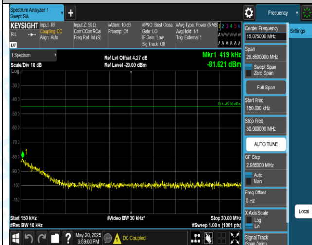
Band38-10MHz-16QAM-37800-1RB#0-0.15~30-PASS
