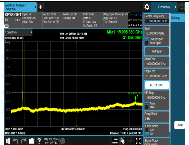
Band38-10MHz-QPSK-38200-1RB#0-1000~20000-PASS
