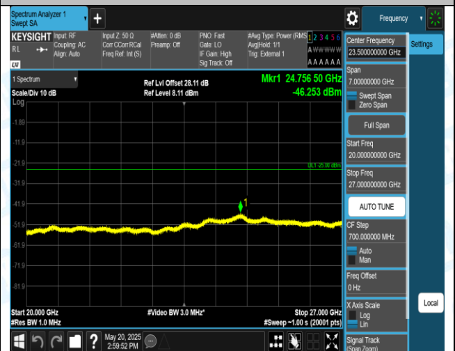
Band38-20MHz-16QAM-38150-1RB#0-20000-27000-PASS
