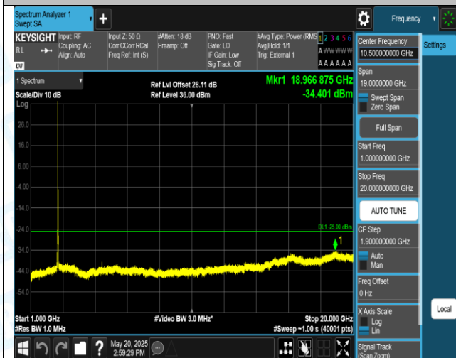
Band38-20MHz-16QAM-38150-1RB#0-1000-20000-PASS
