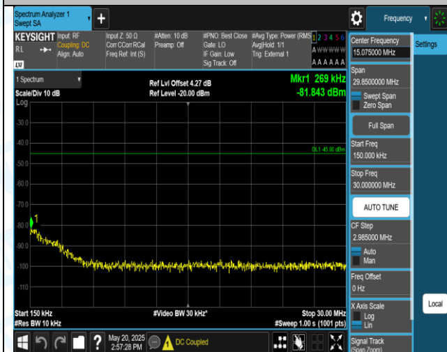
Band38-20MHz-16QAM-38150-1RB#0-0.15-30-PASS
