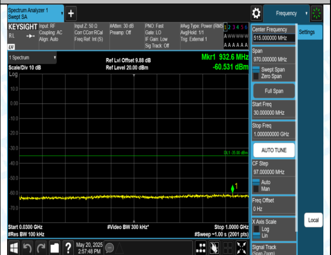
Band38-20MHz-16QAM-38150-1RB#0-30-1000-PASS
