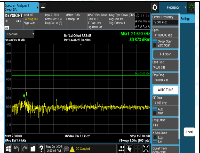
Band38-20MHz-16QAM-38150-1RB#0-0.009-0.15-PASS
