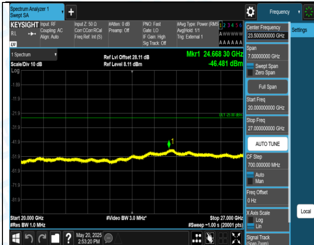
Band38-20MHz-16QAM-38000-1RB#0-20000-27000-PASS
