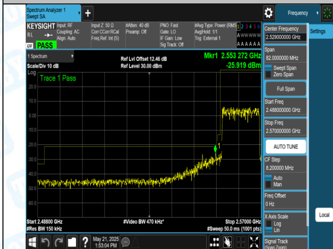
41(2555-2655)-15MHz-16QAM-40315-75RB#0-PASS
