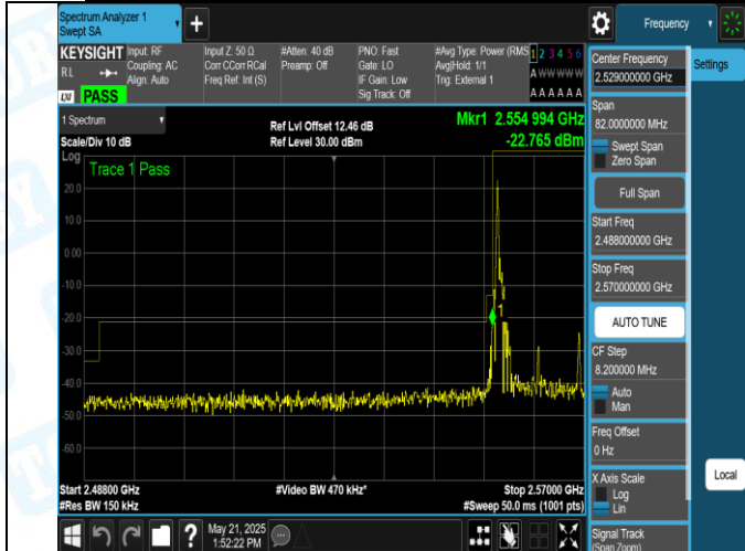
41(2555-2655)-15MHz-16QAM-40315-1RB#0-PASS
