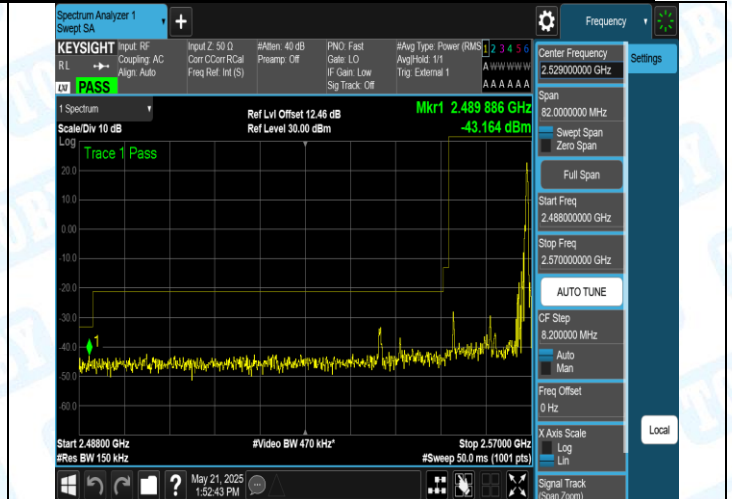
41(2555-2655)-15MHz-16QAM-40315-1RB#74-PASS
