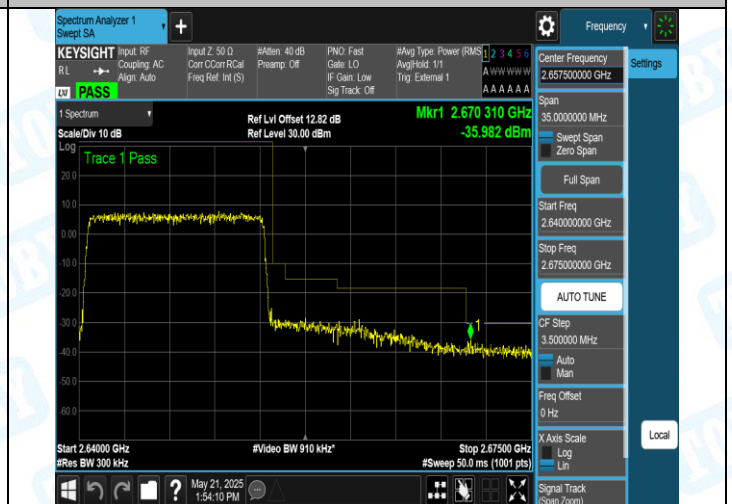
41(2555-2655)-15MHz-16QAM-41165-75RB#0-PASS
