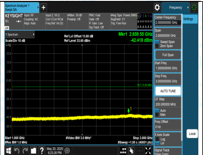
Band5-3MHz-QPSK-20635-1RB#0-1000~3000-PASS
