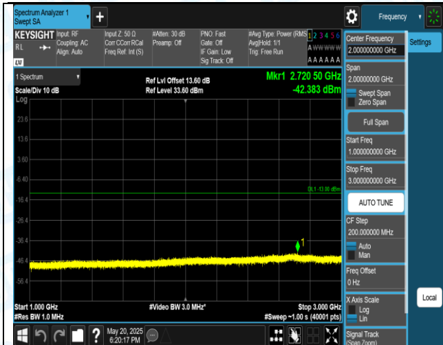
Band5-3MHz-16QAM-20415-1RB#0-1000~3000-PASS
