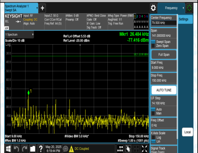
Band5-3MHz-16QAM-20415-1RB#0-0.009~0.15-PASS
