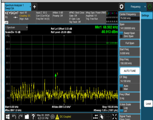
Band5-3MHz-16QAM-20525-1RB#0-0.009~0.15-PASS
