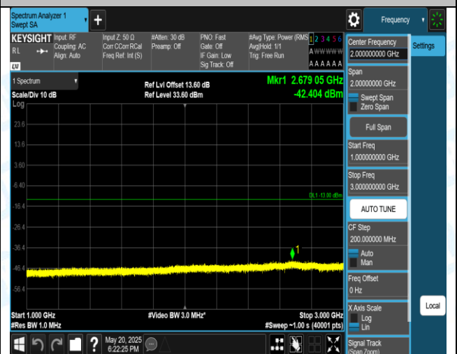
Band5-3MHz-16QAM-20525-1RB#0-1000~3000-PASS
