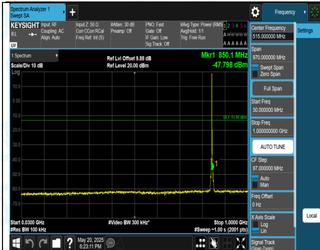
Band5-3MHz-QPSK-20635-1RB#0-30~1000-PASS
