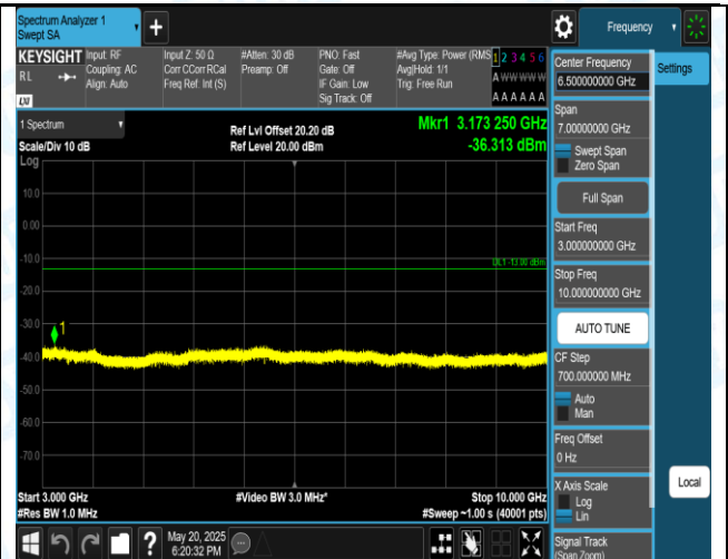
Band5-3MHz-16QAM-20415-1RB#0-3000~10000-PASS
