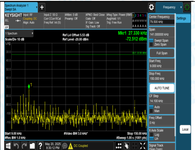
Band5-1.4MHz-16QAM-20643-1RB#0-0.009~0.15-PASS
