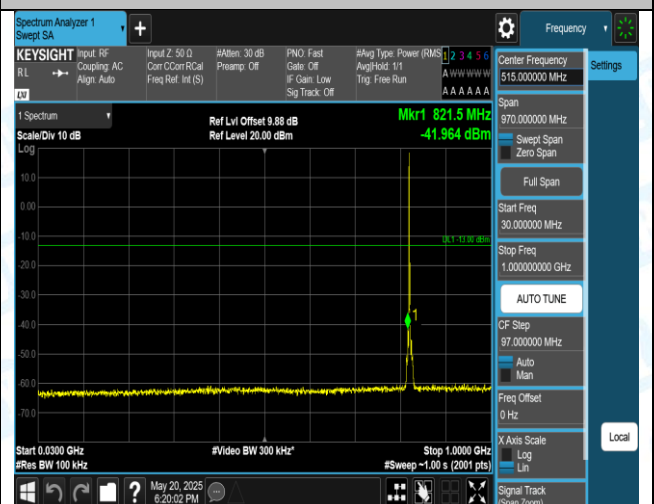
Band5-3MHz-16QAM-20415-1RB#0-30~1000-PASS
