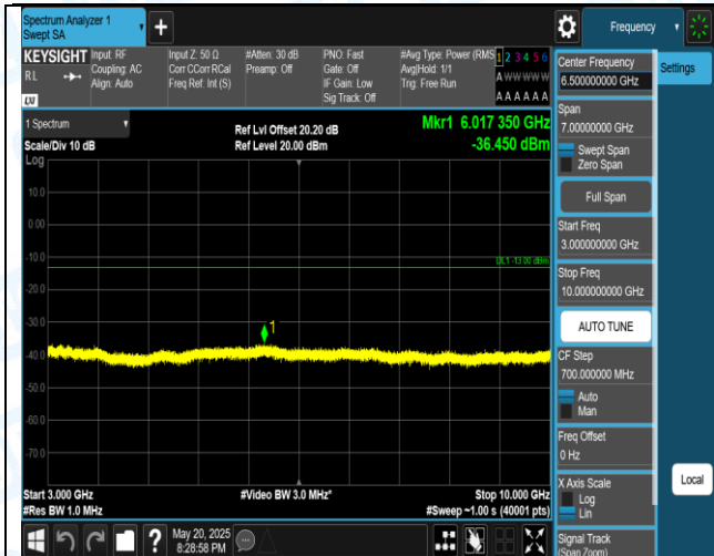
Band5-1.4MHz-16QAM-20525-1RB#0-3000~10000-PASS
