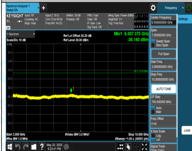
Band5-3MHz-QPSK-20635-1RB#0-3000~10000-PASS
