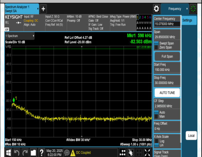
Band5-3MHz-16QAM-20525-1RB#0-0.15~30-PASS
