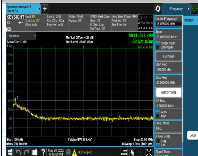
Band5-3MHz-16QAM-20415-1RB#0-0.15~30-PASS
