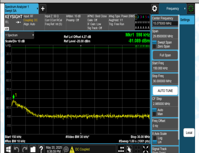
Band5-10MHz-QPSK-20600-1RB#0-0.15~30-PASS
