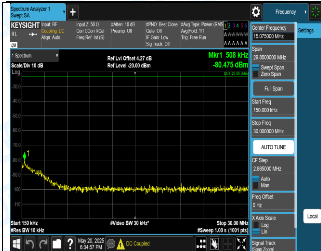
Band5-10MHz-QPSK-20525-1RB#0-0.15~30-PASS
