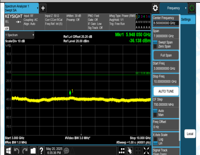
Band5-10MHz-QPSK-20525-1RB#0-3000~10000-PASS
