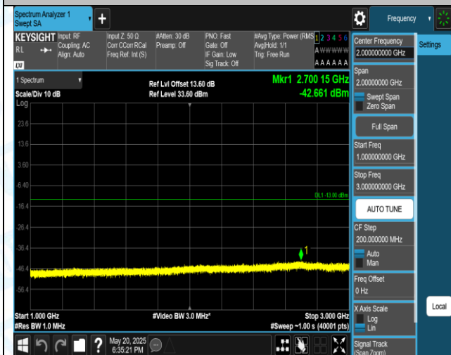
Band5-10MHz-QPSK-20525-1RB#0-1000~3000-PASS
