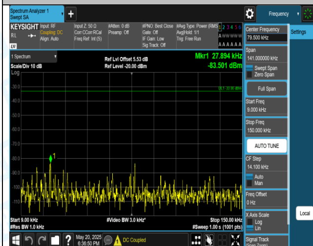
Band5-10MHz-QPSK-20600-1RB#0-0.009~0.15-PASS
