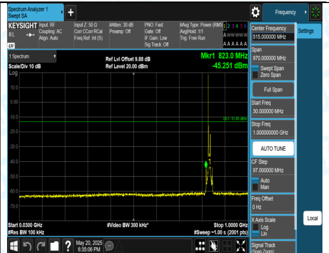
Band5-10MHz-QPSK-20525-1RB#0-30~1000-PASS
