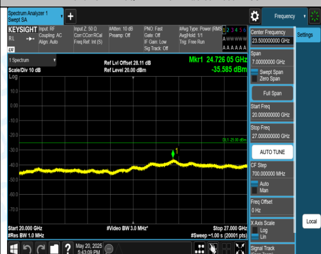
Band7-5MHz-16QAM-21425-1RB#0-20000~27000-PASS
