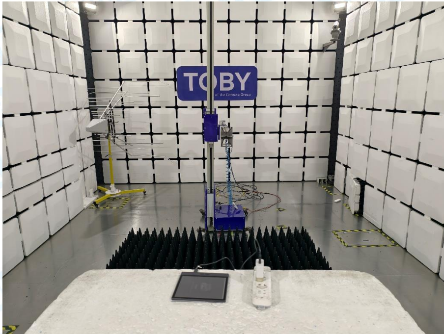
Photo of Setup for Radiated Emission (Above 1 GHz)----BT&WIFI
