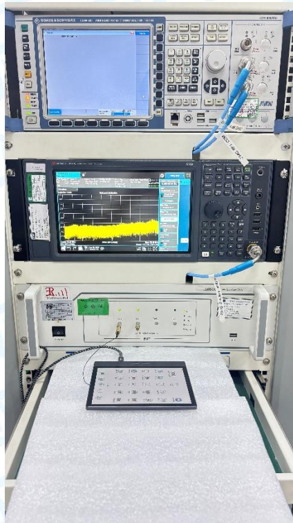
Photo of Setup for RF Conducted----GSM&WCDMA&LTE
