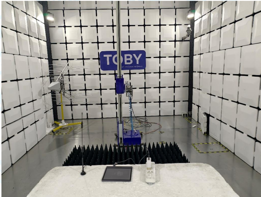
Photo of Setup for Radiated Emission (Above 1 GHz)----GSM&WCDMA&LTE
