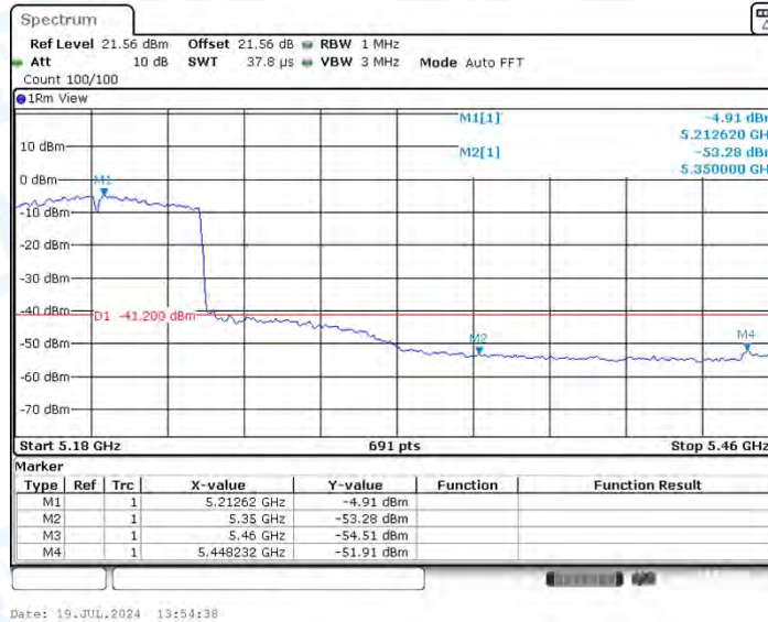
11AC80SISO_Ant1_High_5210_Peak
