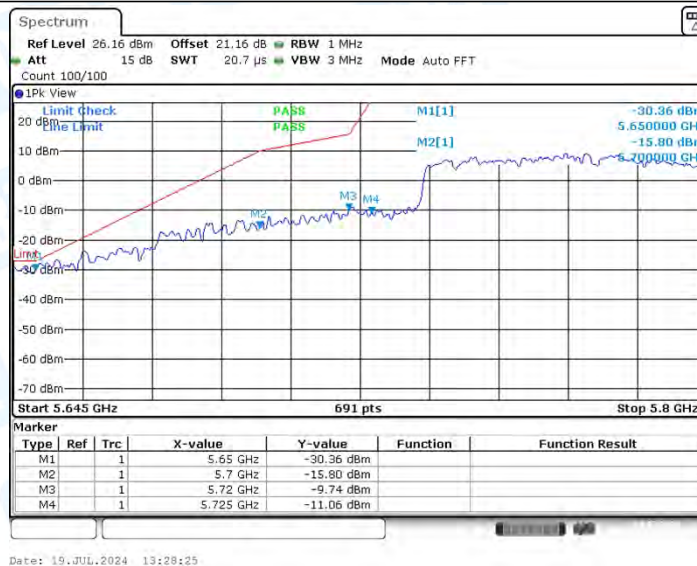
11AC80SISO_Ant1_High_5775_Peak
