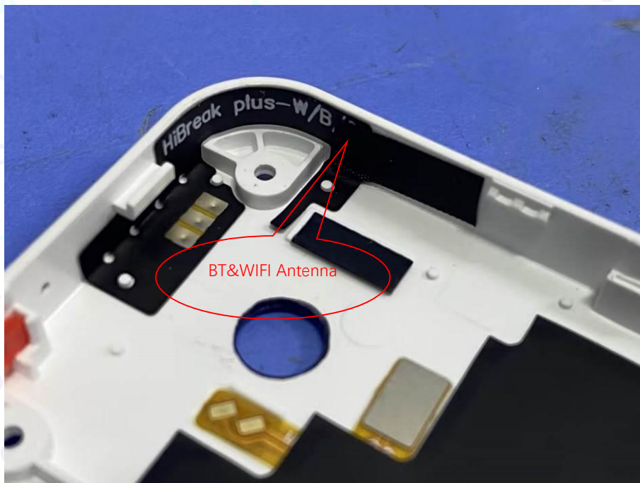
Photo 13 Internal of Antenna
