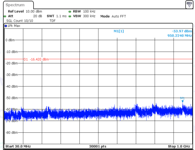
DH5-Ant1-2402-30~1000-PASS
