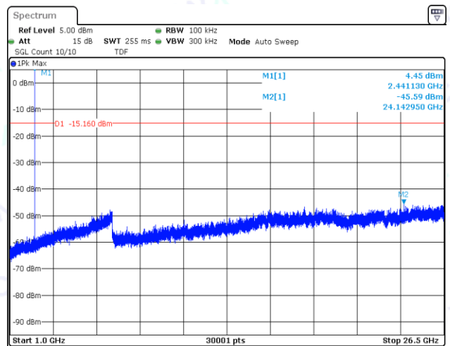
DH5-Ant1-2441-0~Reference-PASS
