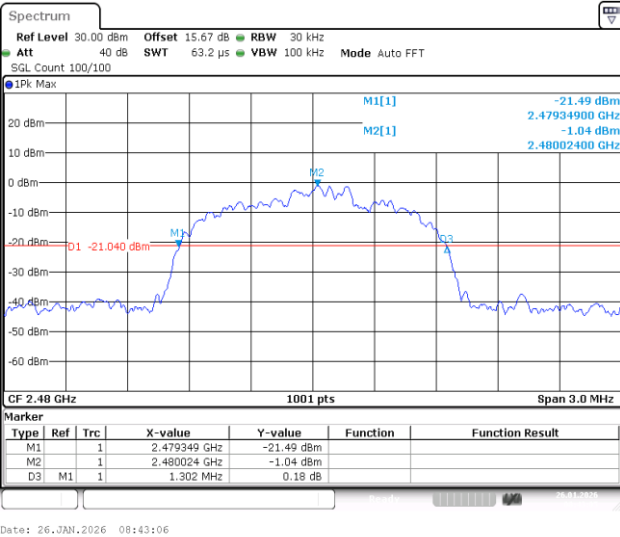
3DH5-Ant1-2480
