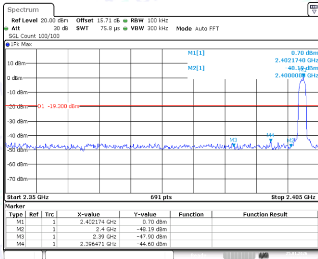
DH5-Ant1-Hop_2402-PASS
