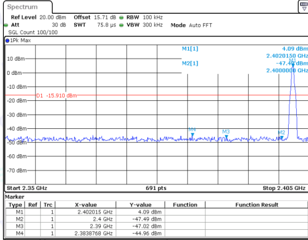
DH5-Ant1-2402-PASS
