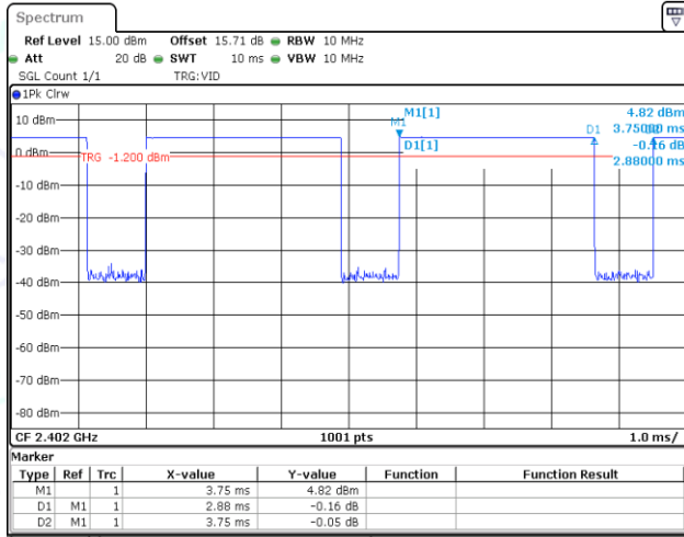
NTNV-DH5-Ant1-2402
