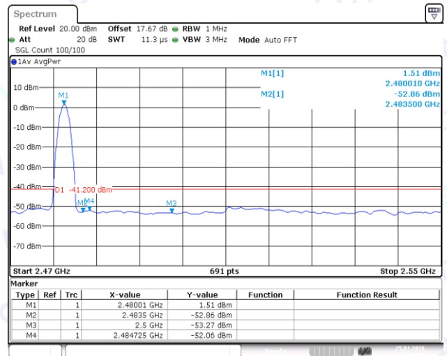
2DH5-Ant1-2480-PASS
