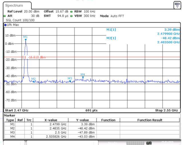
DH5-Ant1-Hop_2480-PASS
