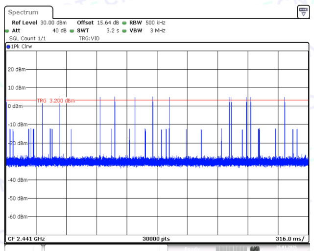
2DH1-Ant1-Hop-PASS
