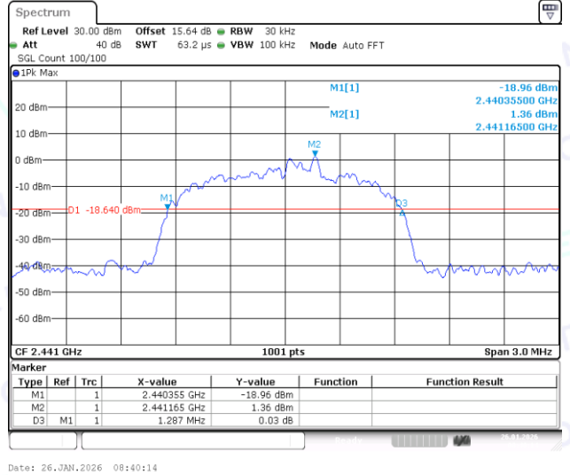
3DH5-Ant1-2441
