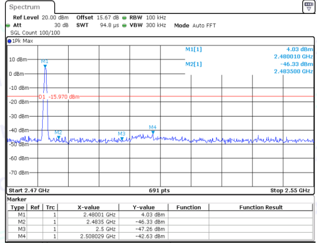
DH5-Ant1-2480-PASS
