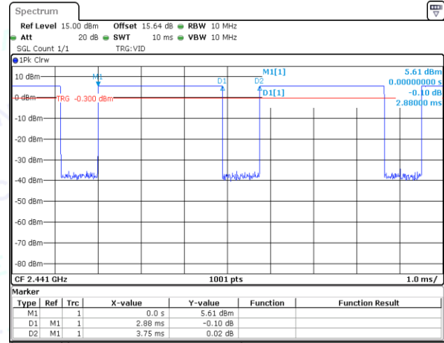
NTNV-DH5-Ant1-2441
