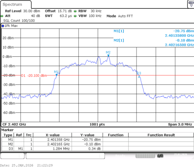
3DH5-Ant1-2402
