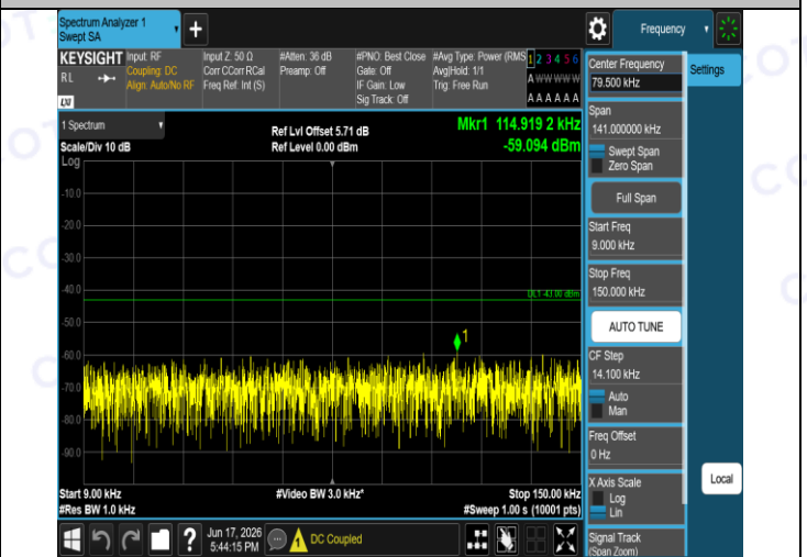
Band2-9400-4-0.009~0.15MHz-PASS
