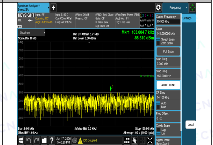
Band2-9538-4-0.009~0.15MHz-PASS
