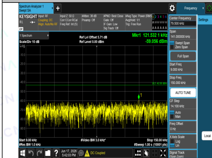
Band2-9538-3-0.009~0.15MHz-PASS
