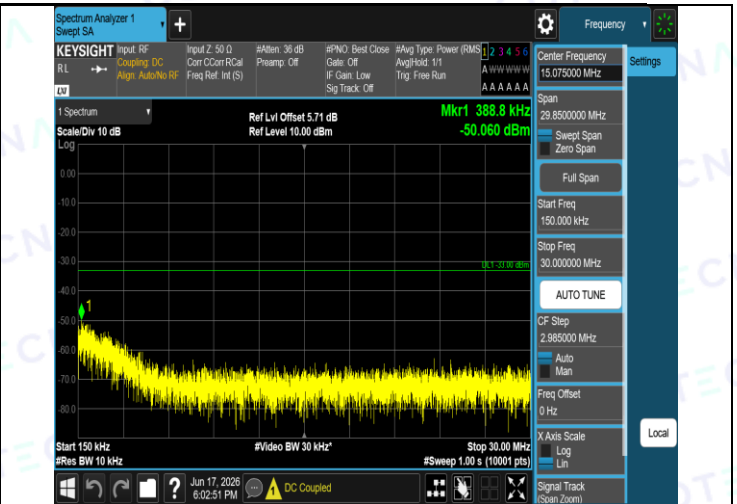
Band2-9262-5-0.15~30MHz-PASS
