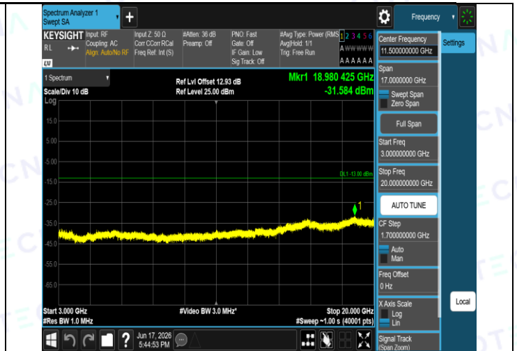
Band2-9400-4-3000~20000MHz-PASS
