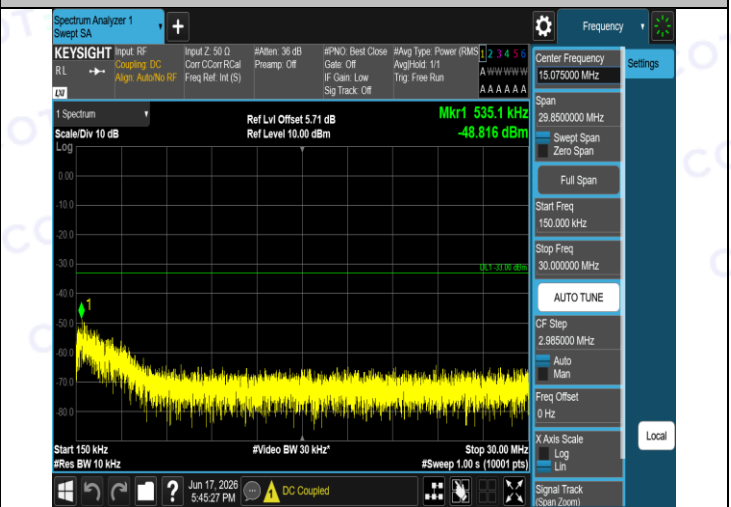
Band2-9538-4-0.15~30MHz-PASS
