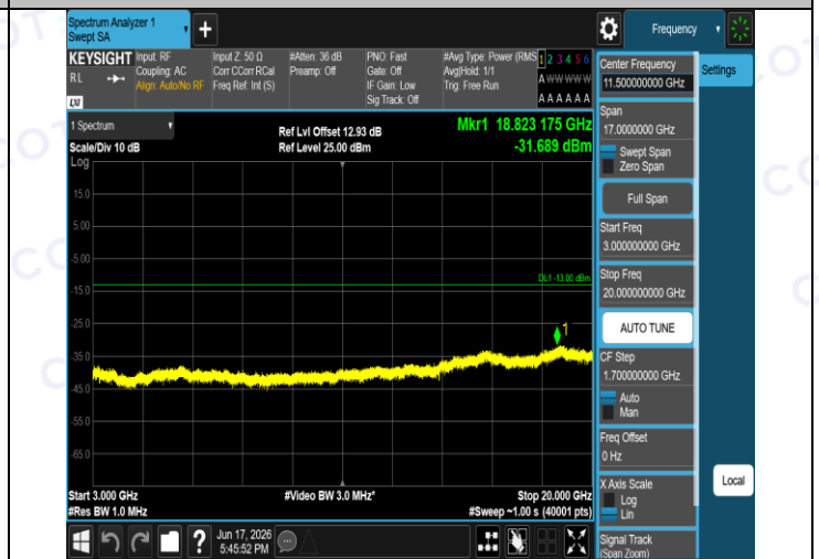
Band2-9538-4-3000~20000MHz-PASS
