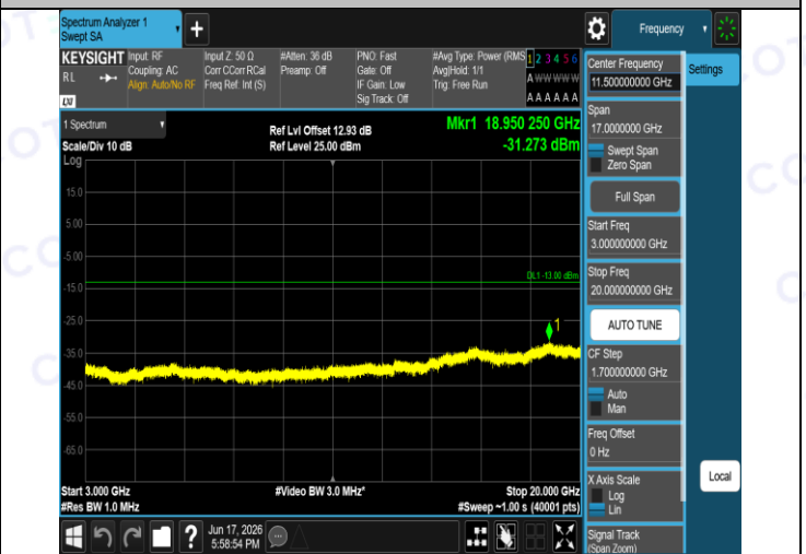
Band2-9262-4-3000~20000MHz-PASS
