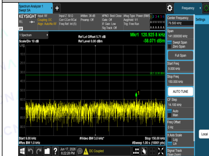
Band5-4182-3-0.009~0.15MHz-PASS
