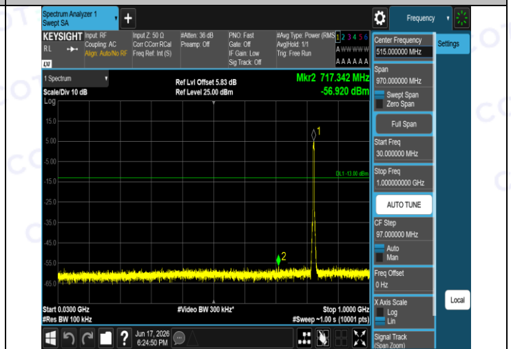
Band5-4132-4-30~1000MHz-PASS
