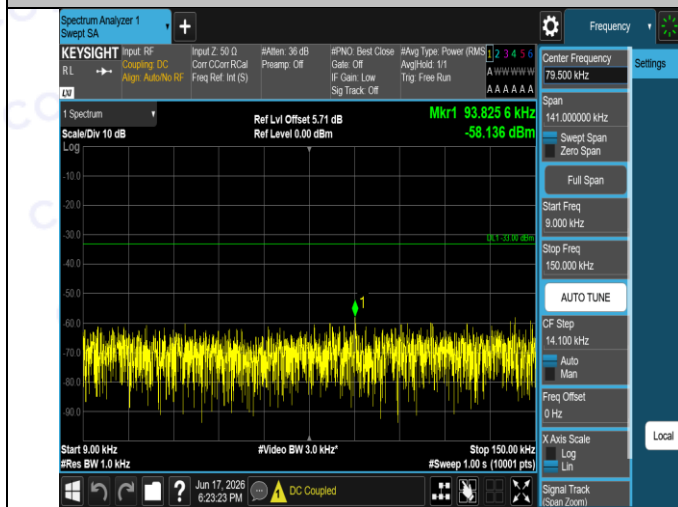
Band5-4233-3-0.009~0.15MHz-PASS
