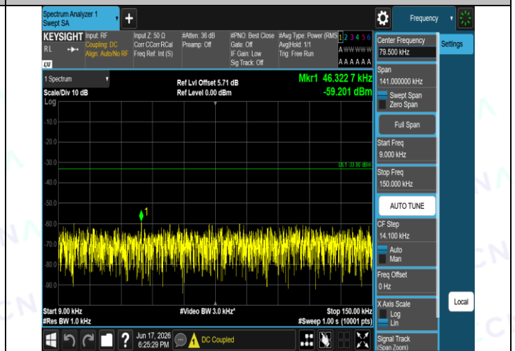
Band5-4182-4-0.009~0.15MHz-PASS
