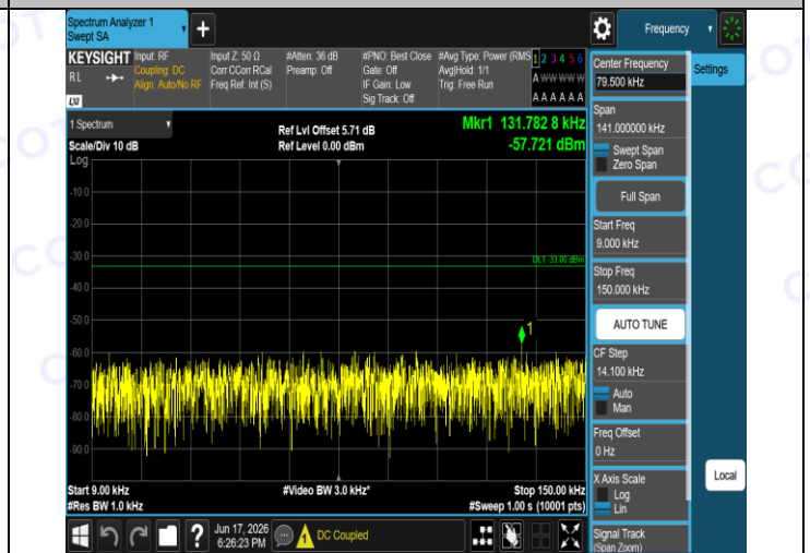
Band5-4233-4-0.009~0.15MHz-PASS
