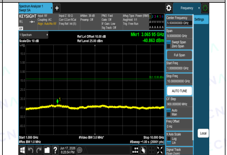
Band5-4182-4-1000~10000MHz-PASS
