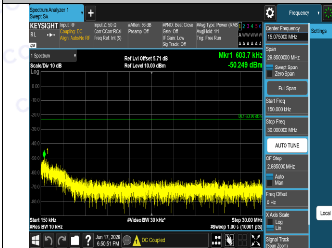
Band5-4182-4-0.15~30MHz-PASS
