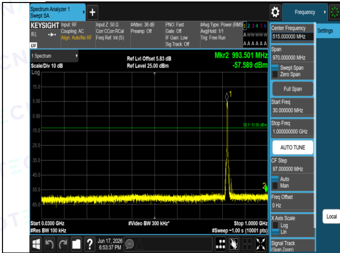
Band5-4132-5-30~1000MHz-PASS
