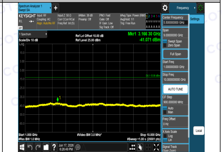
Band5-4233-4-1000~10000MHz-PASS
