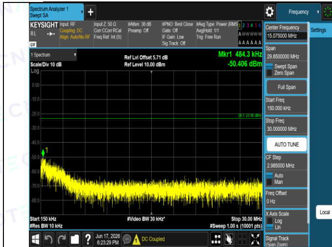
Band5-4233-3-0.15~30MHz-PASS
