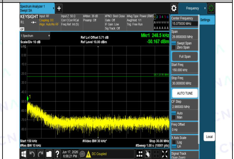
Band5-4233-5-0.15~30MHz-PASS
