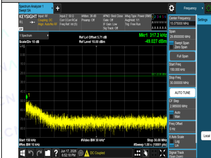
Band5-4233-4-0.15~30MHz-PASS
