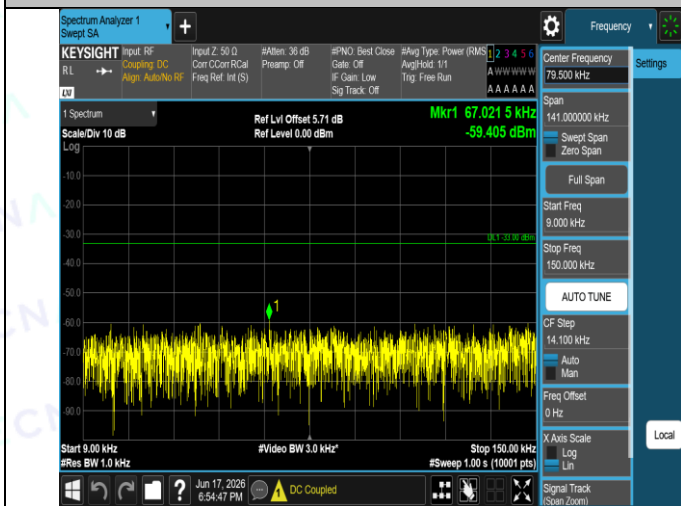
Band5-4182-5-0.009~0.15MHz-PASS
