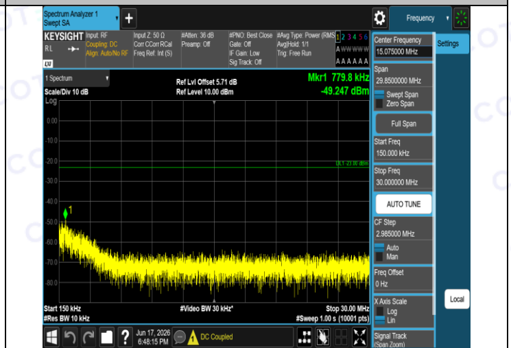
Band5-4233-3-0.15~30MHz-PASS
