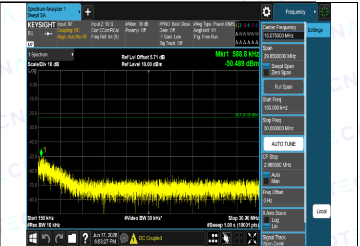
Band5-4132-5-0.15~30MHz-PASS
