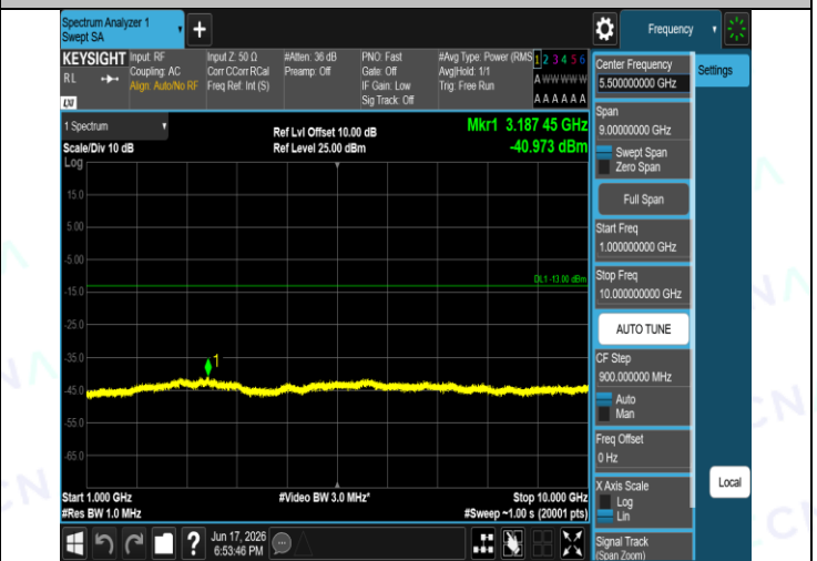
Band5-4132-5-1000~10000MHz-PASS
