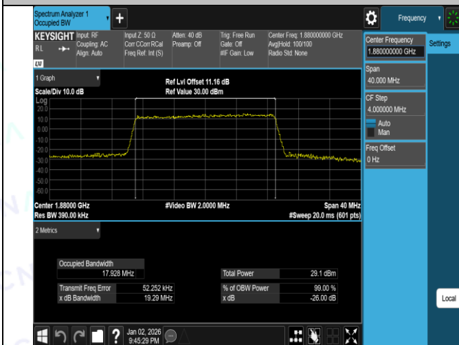
Band2-20MHz-16QAM-18900-100RB#0-PASS
