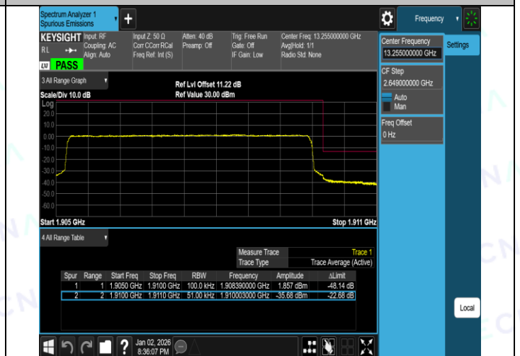
Band2-5MHz-16QAM-18625-1RB#24-PASS
