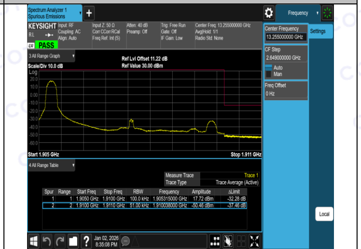
Band2-5MHz-QPSK-19175-25RB#0-PASS
