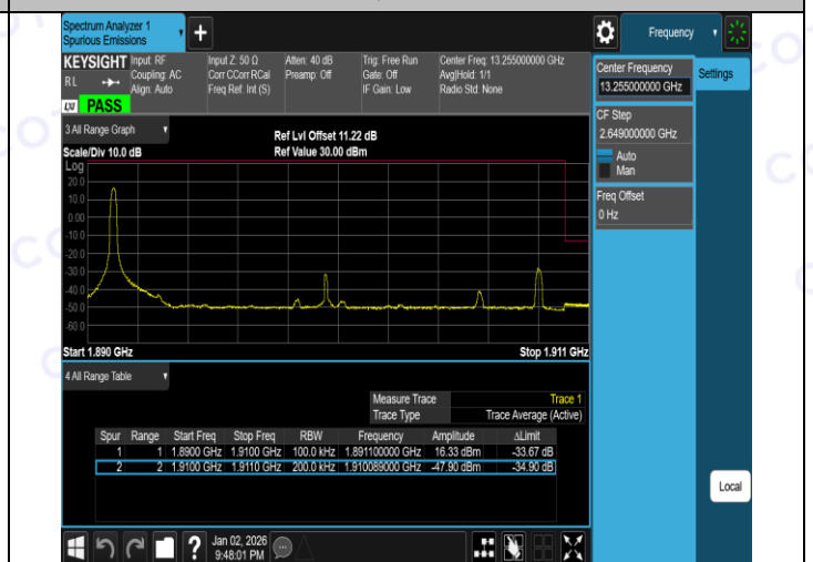
Band2-20MHz-16QAM-19100-100RB#0-PASS
