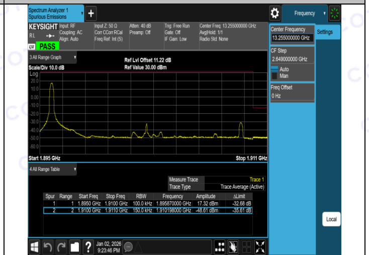
Band2-15MHz-QPSK-19125-75RB#0-PASS
