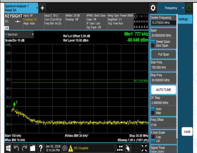
Band2-3MHz-QPSK-19185-1RB#0-1000~3000-PASS
