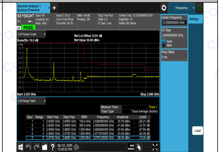
Band41(2535-2655)-20MHz-16QAM-41140-100RB#0-PASS
