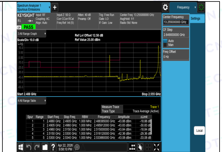
Band41(2535-2655)-20MHz-16QAM-41140-1RB#0-PASS
