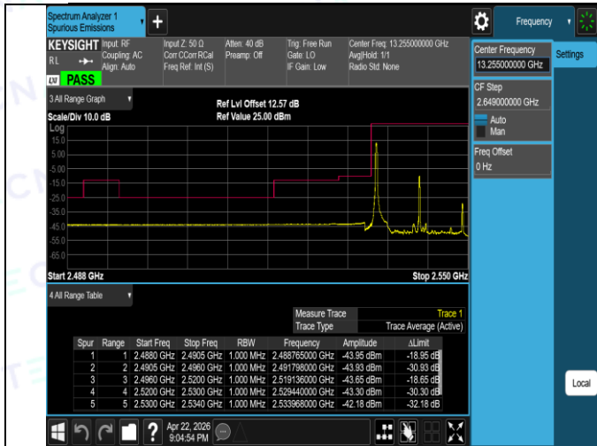
Band41(2535-2655)-15MHz-QPSK-40115-75RB#0-PASS
