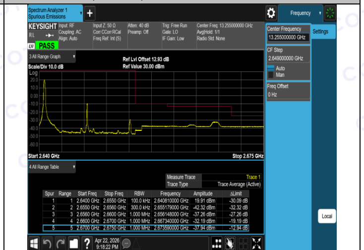
Band41(2535-2655)-15MHz-16QAM-41165-75RB#0-PASS
