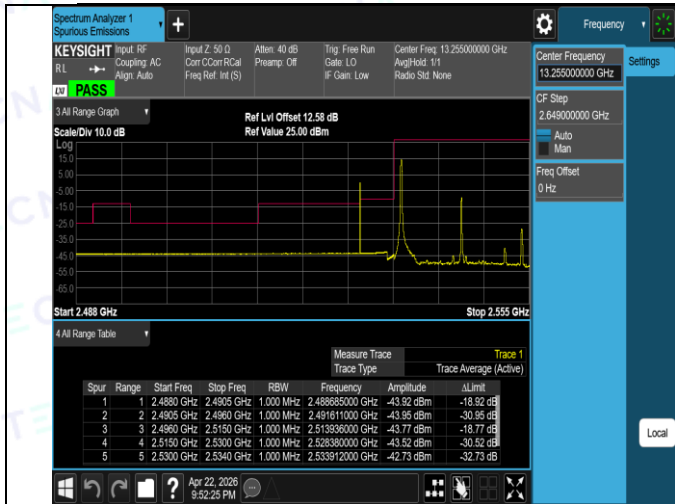
Band41(2535-2655)-20MHz-QPSK-40140-100RB#0-PASS
