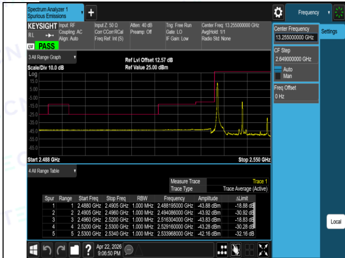
Band41(2535-2655)-15MHz-16QAM-40115-75RB#0-PASS
