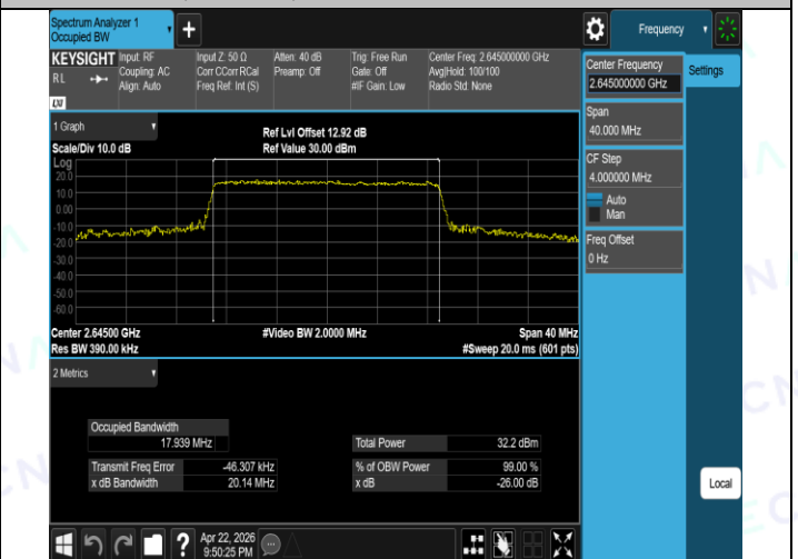
Band41(2535-2655)-20MHz-16QAM-41140-100RB#0-PASS
