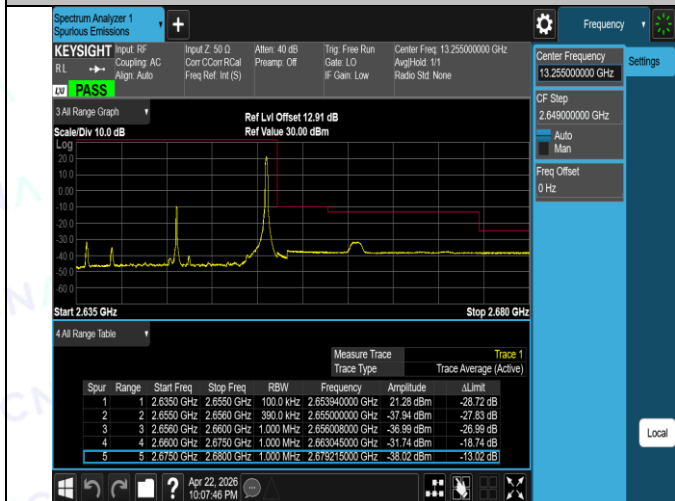
Band41(2535-2655)-20MHz-16QAM-40140-1RB#0-PASS
