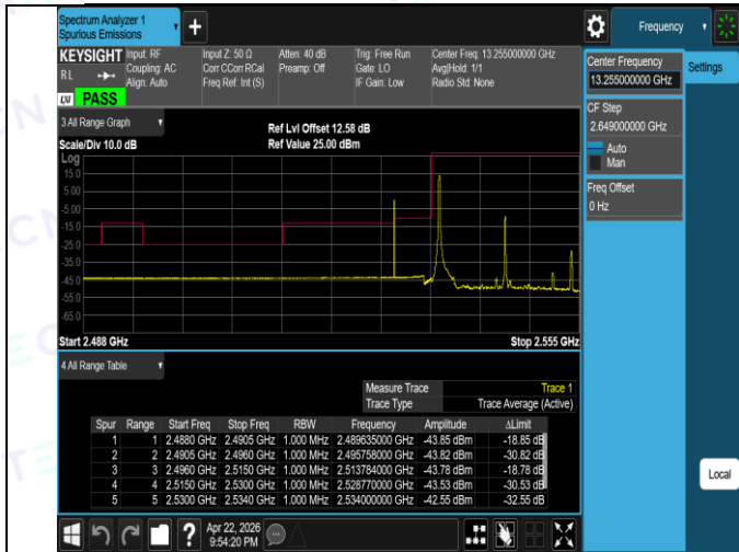
Band41(2535-2655)-20MHz-16QAM-40140-100RB#0-PASS
