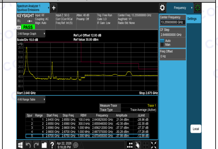
Band41(2535-2655)-15MHz-QPSK-41165-75RB#0-PASS
