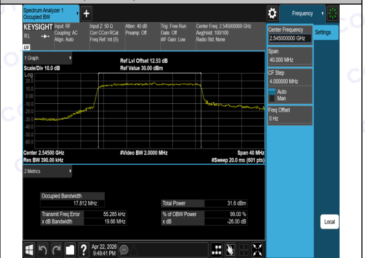
Band41(2535-2655)-20MHz-16QAM-41140-100RB#0-PASS
