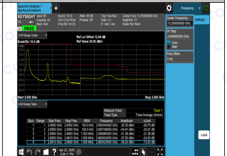
Band41(2535-2655)-5MHz-16QAM-41215-25RB#0-PASS
