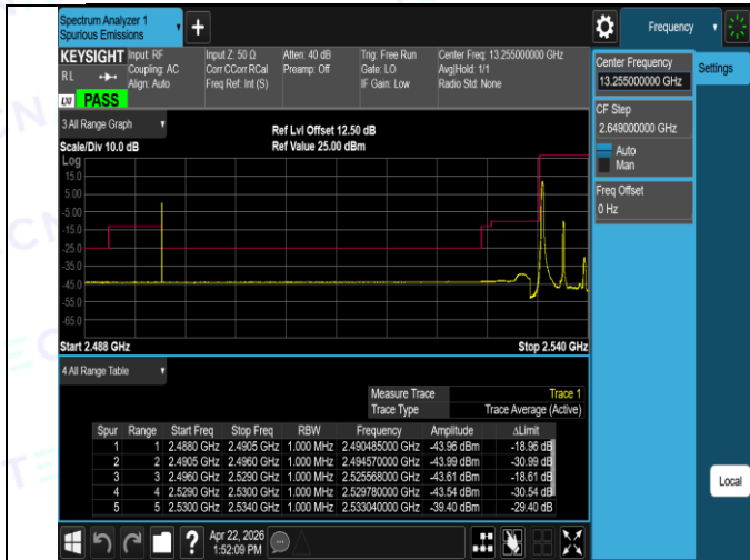
Band41(2535-2655)-5MHz-16QAM-40065-25RB#0-PASS
