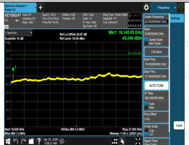
Band41(2535-2655)-5MHz-16QAM-41215-1RB#0-0.15~30-PASS
