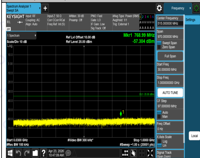
Band41(2535-2655)-10MHz-16QAM-41190-1RB#0-3000~18000-PASS
