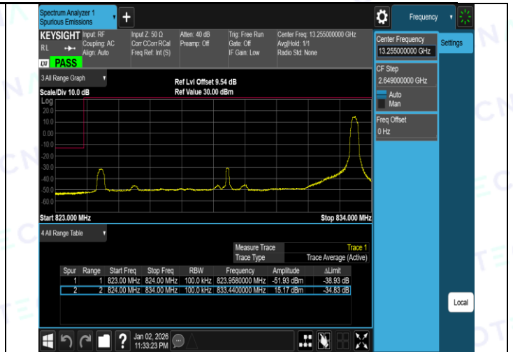
Band5-10MHz-16QAM-20600-1RB#0-PASS
