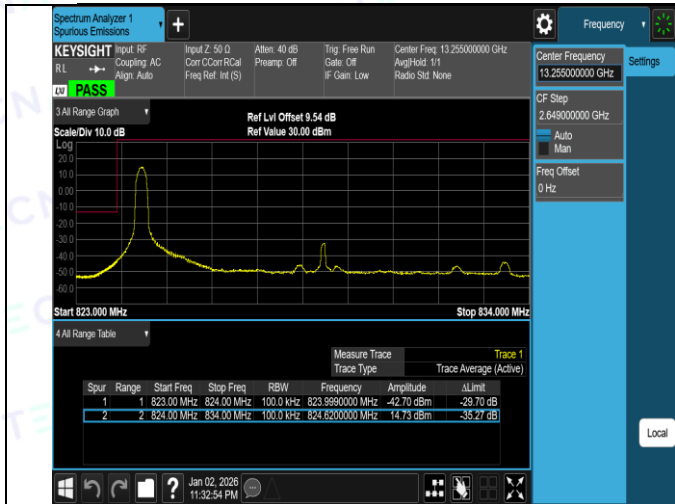
Band5-10MHz-16QAM-20450-50RB#0-PASS
