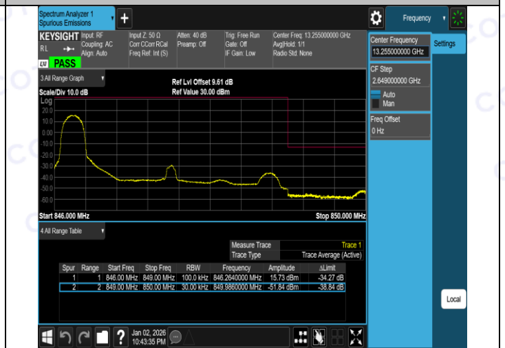
Band5-3MHz-QPSK-20635-15RB#0-PASS
