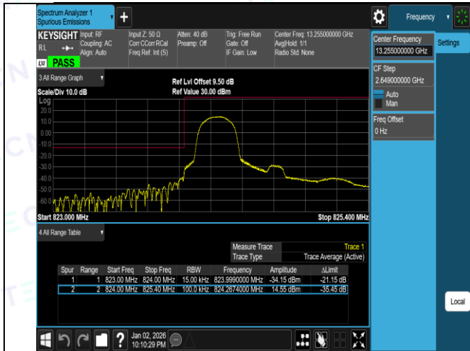
Band5-1.4MHz-16QAM-20407-6RB#0-PASS
