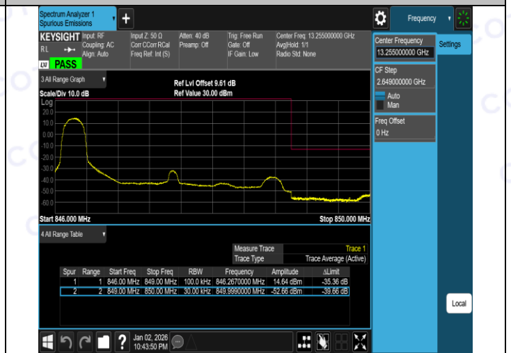
Band5-3MHz-16QAM-20635-15RB#0-PASS
