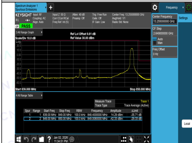
Band5-10MHz-16QAM-20600-1RB#49-PASS
