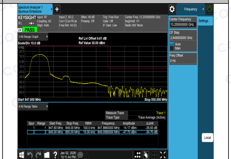
Band5-1.4MHz-16QAM-20643-6RB#0-PASS
