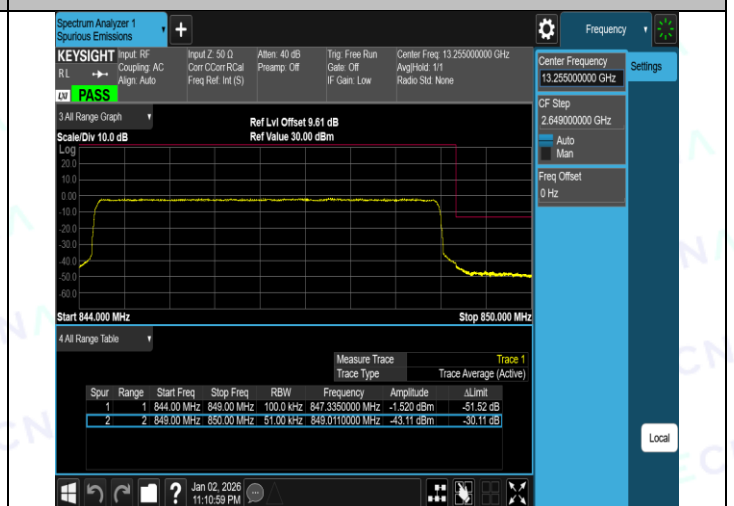
Band5-10MHz-QPSK-20450-1RB#49-PASS
