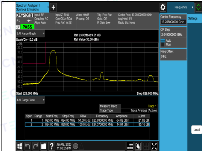
Band5-5MHz-16QAM-20425-25RB#0-PASS
