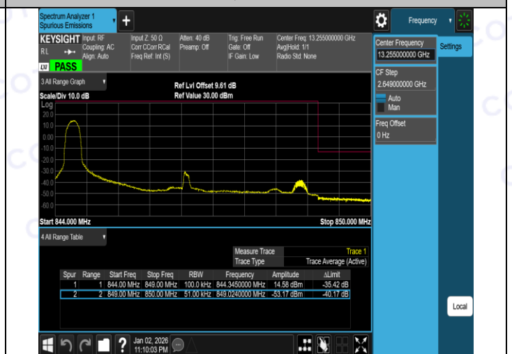
Band5-5MHz-16QAM-20625-25RB#0-PASS
