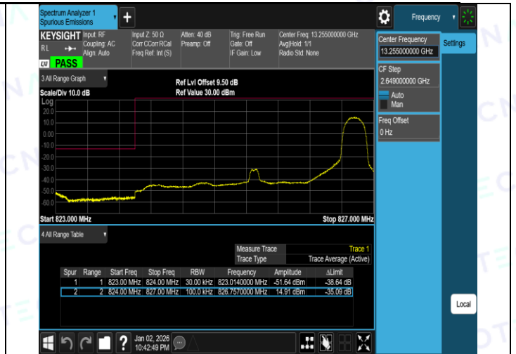
Band5-3MHz-16QAM-20635-1RB#0-PASS
