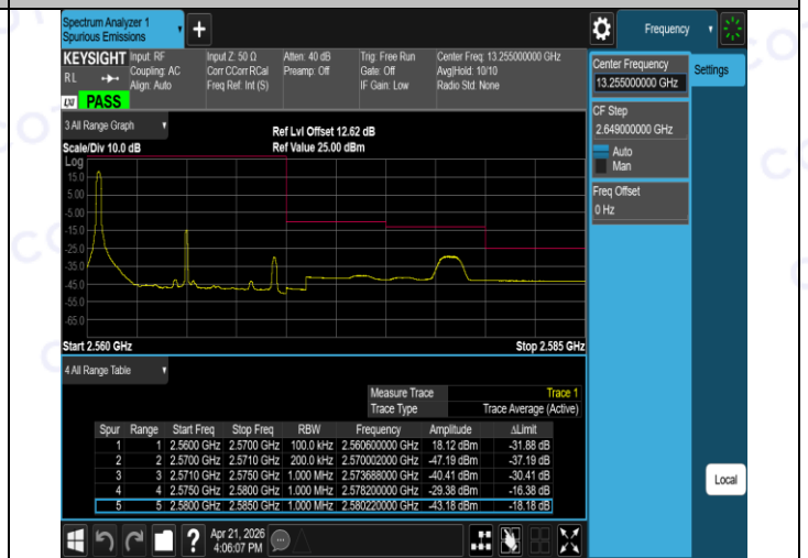
Band7-10MHz-16QAM-21400-50RB#0-PASS
