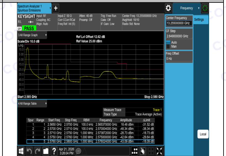
Band7-5MHz-16QAM-21425-25RB#0-PASS
