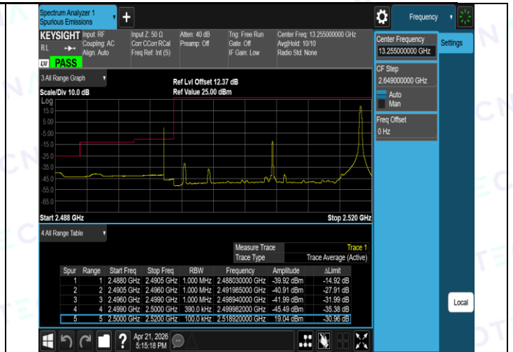
Band7-20MHz-QPSK-21350-1RB#0-PASS
