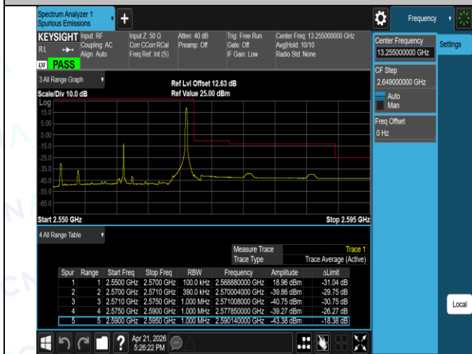
Band7-20MHz-16QAM-20850-1RB#0-PASS
