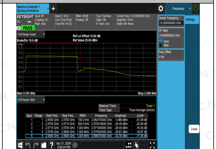
Band7-15MHz-16QAM-20825-1RB#74-PASS
