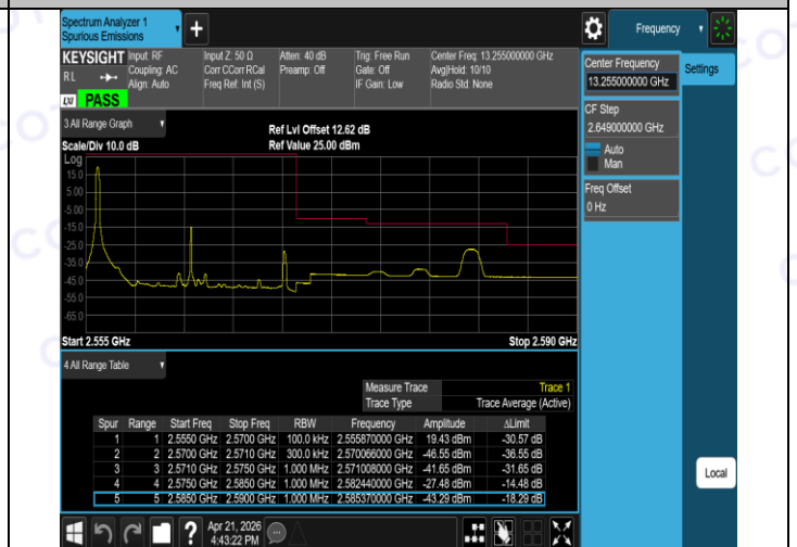
Band7-15MHz-QPSK-21375-75RB#0-PASS
