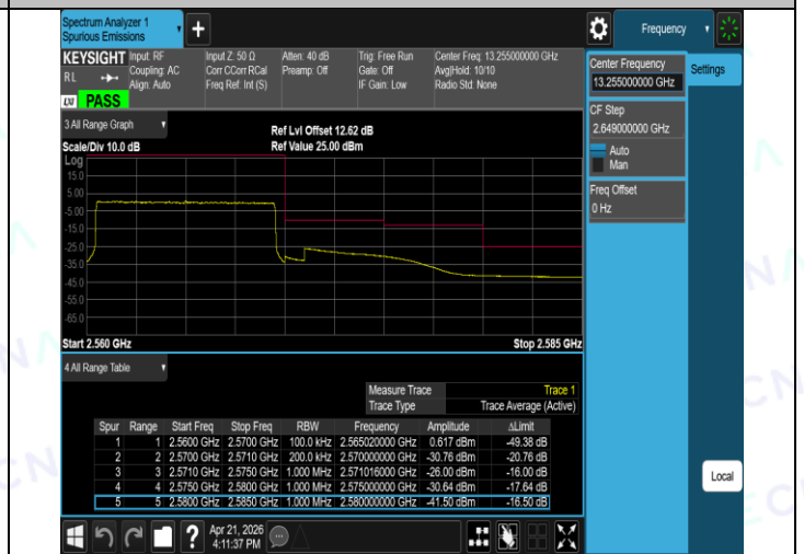
Band7-10MHz-16QAM-20800-1RB#49-PASS
