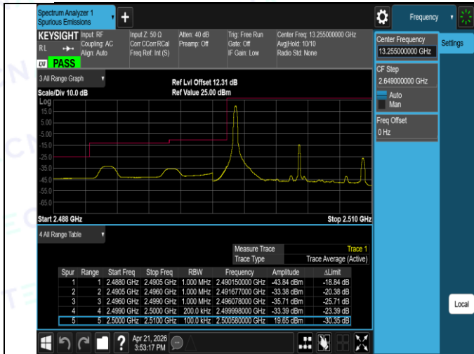
Band7-10MHz-QPSK-20800-50RB#0-PASS
