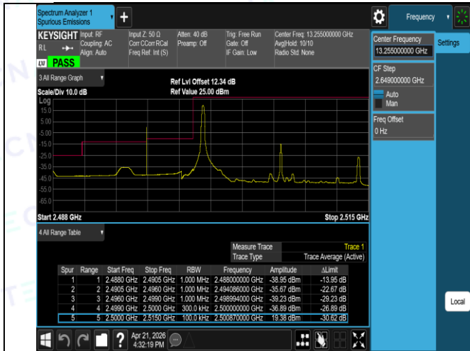
Band7-15MHz-QPSK-20825-75RB#0-PASS
