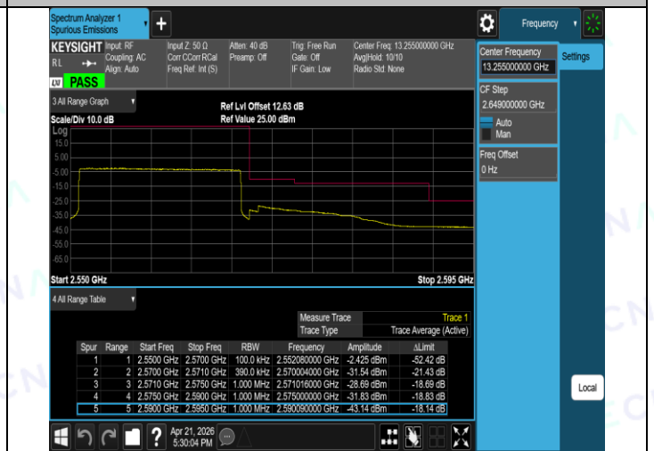
Band7-20MHz-16QAM-20850-1RB#99-PASS
