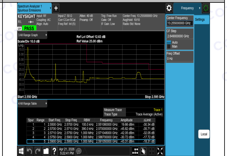
Band7-20MHz-QPSK-21350-100RB#0-PASS
