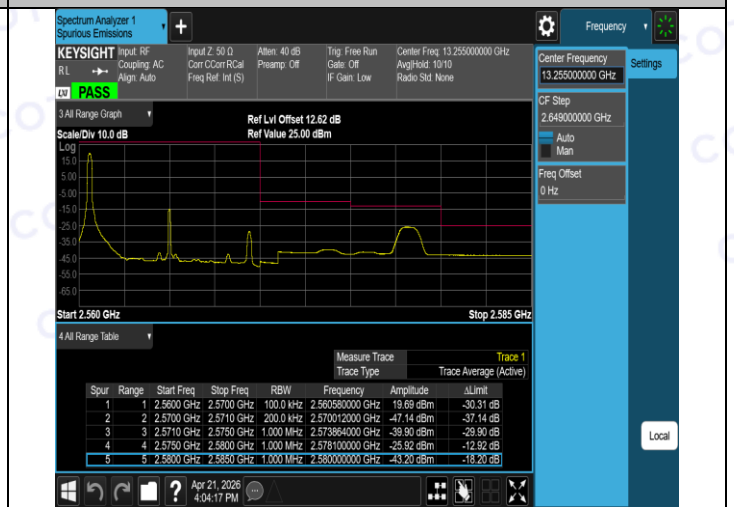
Band7-10MHz-QPSK-21400-50RB#0-PASS
