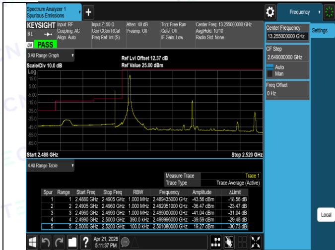
Band7-20MHz-QPSK-20850-100RB#0-PASS
