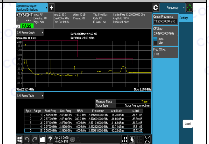
Band7-15MHz-16QAM-21375-75RB#0-PASS
