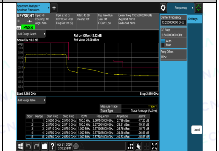
Band7-10MHz-QPSK-20800-1RB#49-PASS
