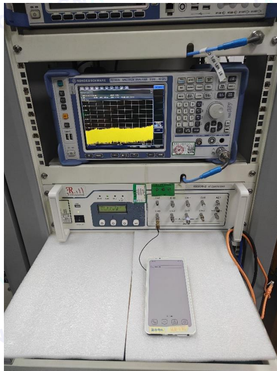
Photo of Setup for RF Conducted----BT&WIFI
