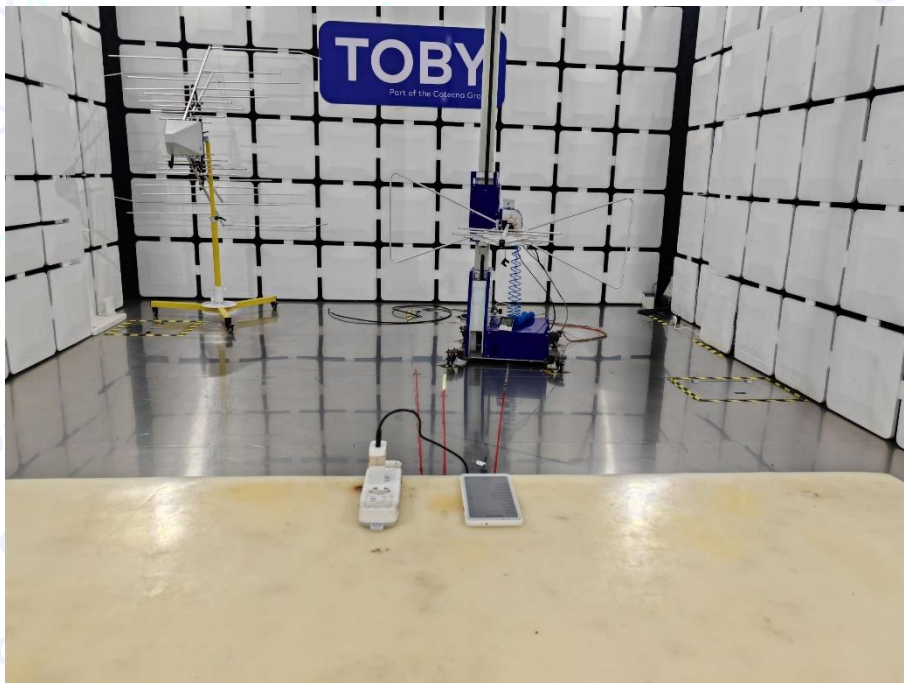
Photo of Setup for Radiated Emission (Below 1 GHz)----BT&WIFI
