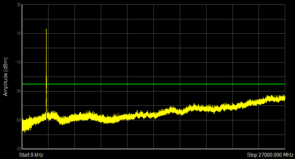
Band7 16QAM BW=20MHz Channel=20850 RB Size=100 Position=#0
