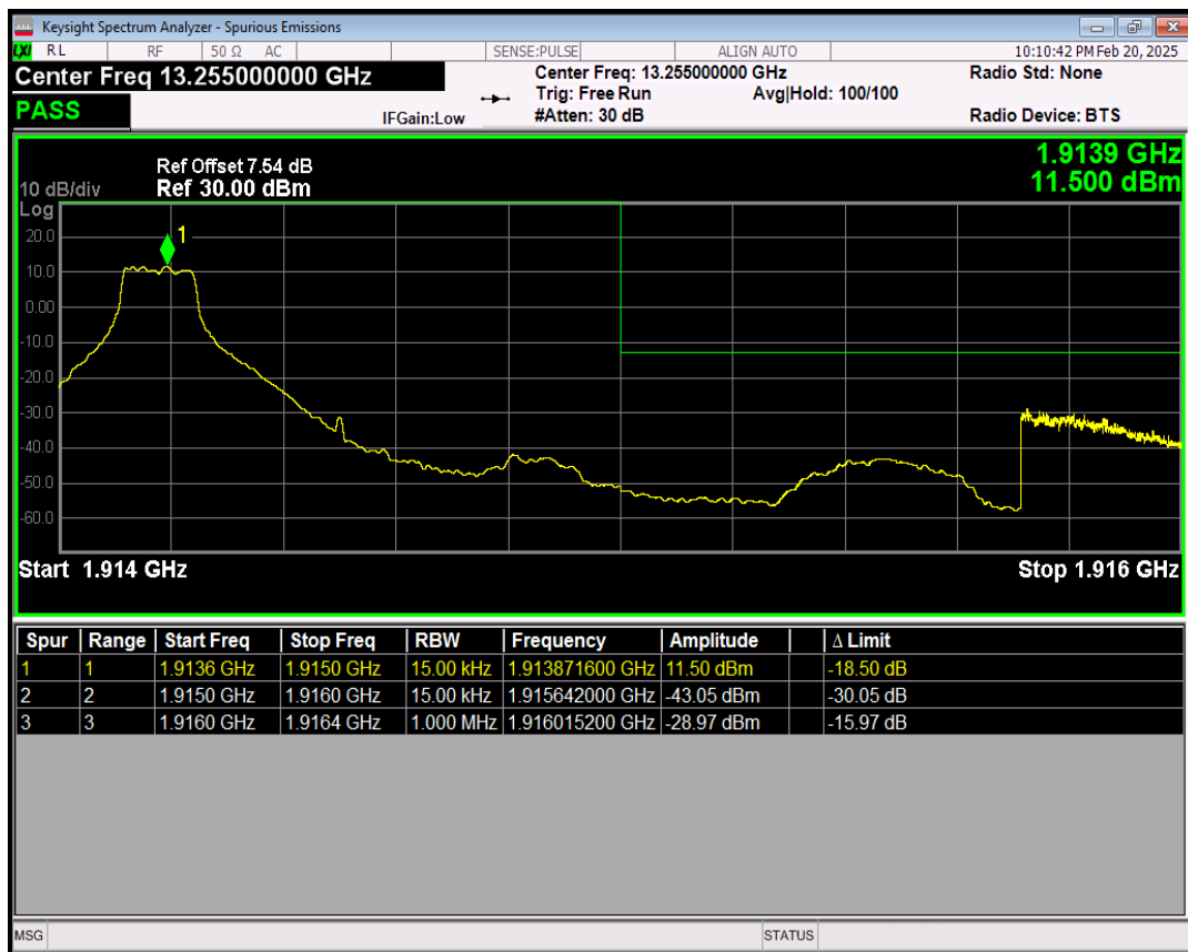
Band25 16QAM BW=1.4MHz Channel=26683 RB Size=1 Position=#Max
