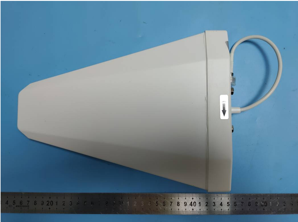
Outdoor Yagi antenna(model: HG-1005)
