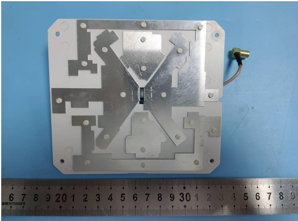
Built-in Antenna
