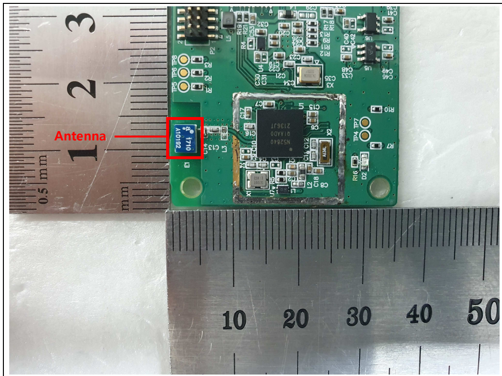
&lt;BLE Antenna&gt;
