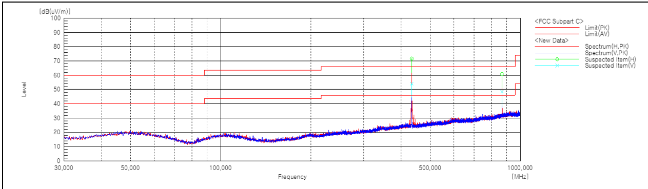
2 nd harmonic
