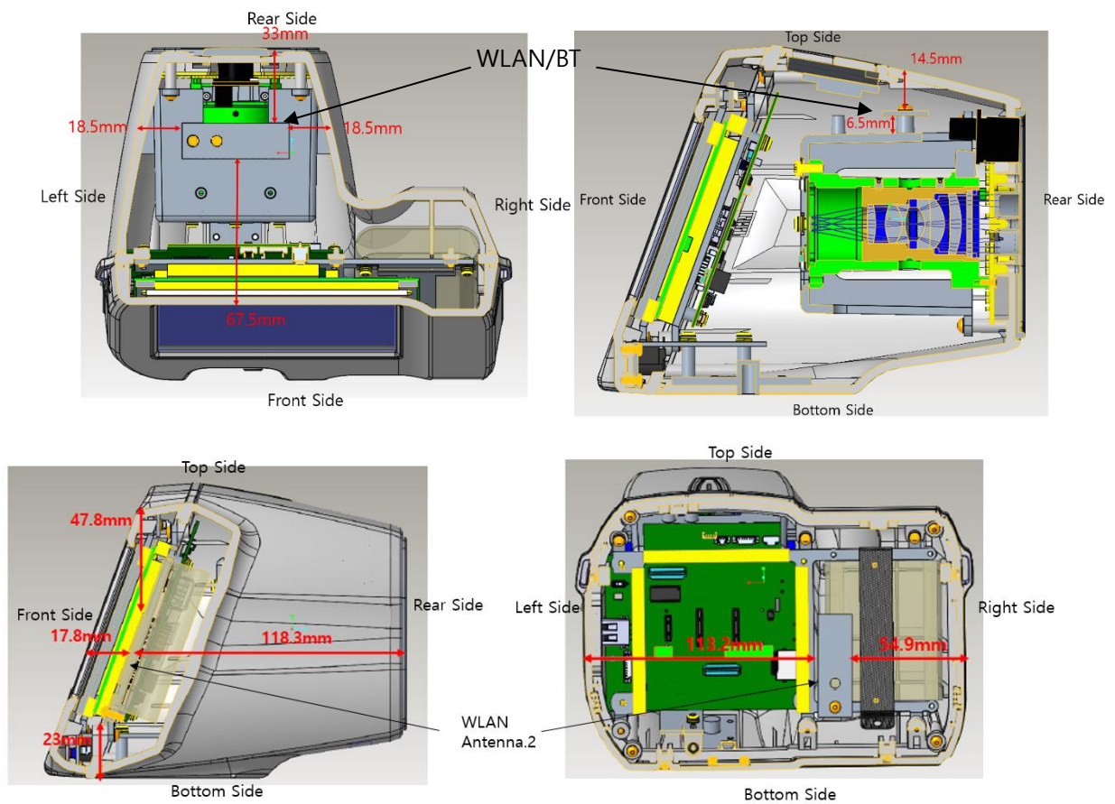
Figure E-1 Antenna Location
