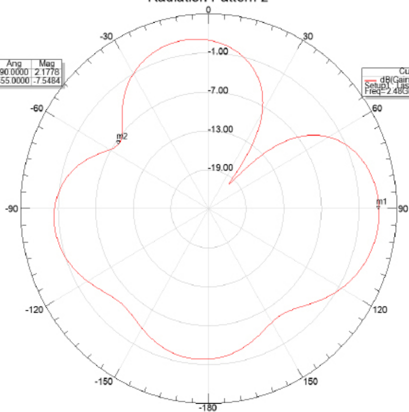
Radiation Pattern 2
