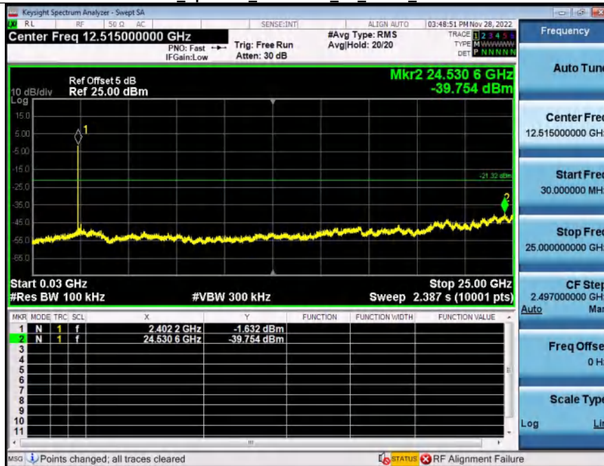
2_Spurious_Emissions_BT_1-DH5_2402
