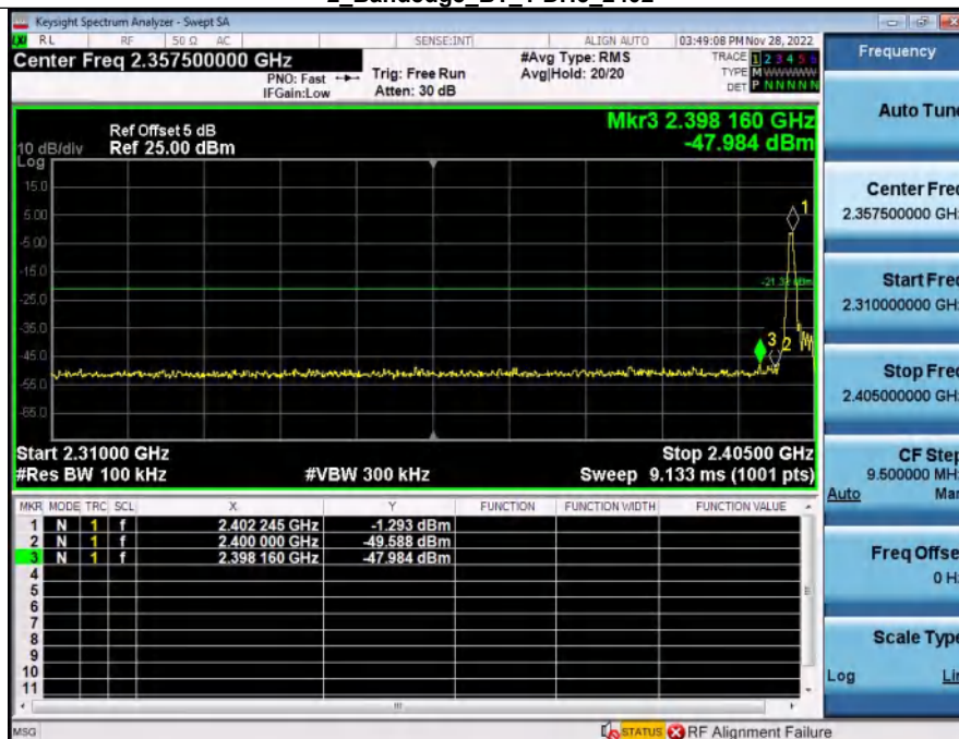
2 Bandedge BT 1-DH5 2402
