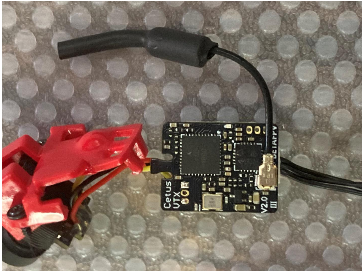
Figure 6. Bottom of radio PCB and Antenna
