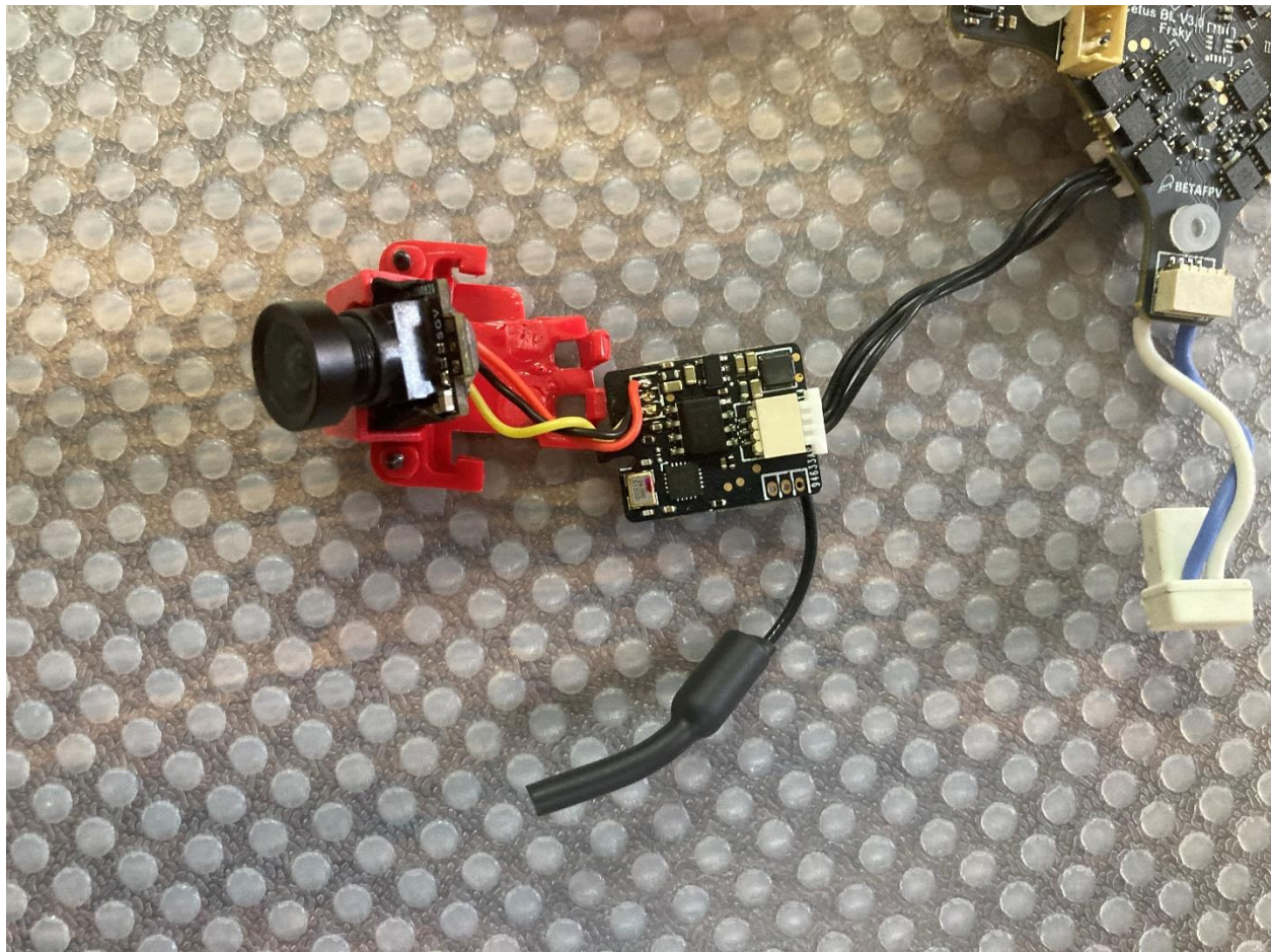
Figure 5. Radio PCB removed from sub-housing (Top of radio PCB)
