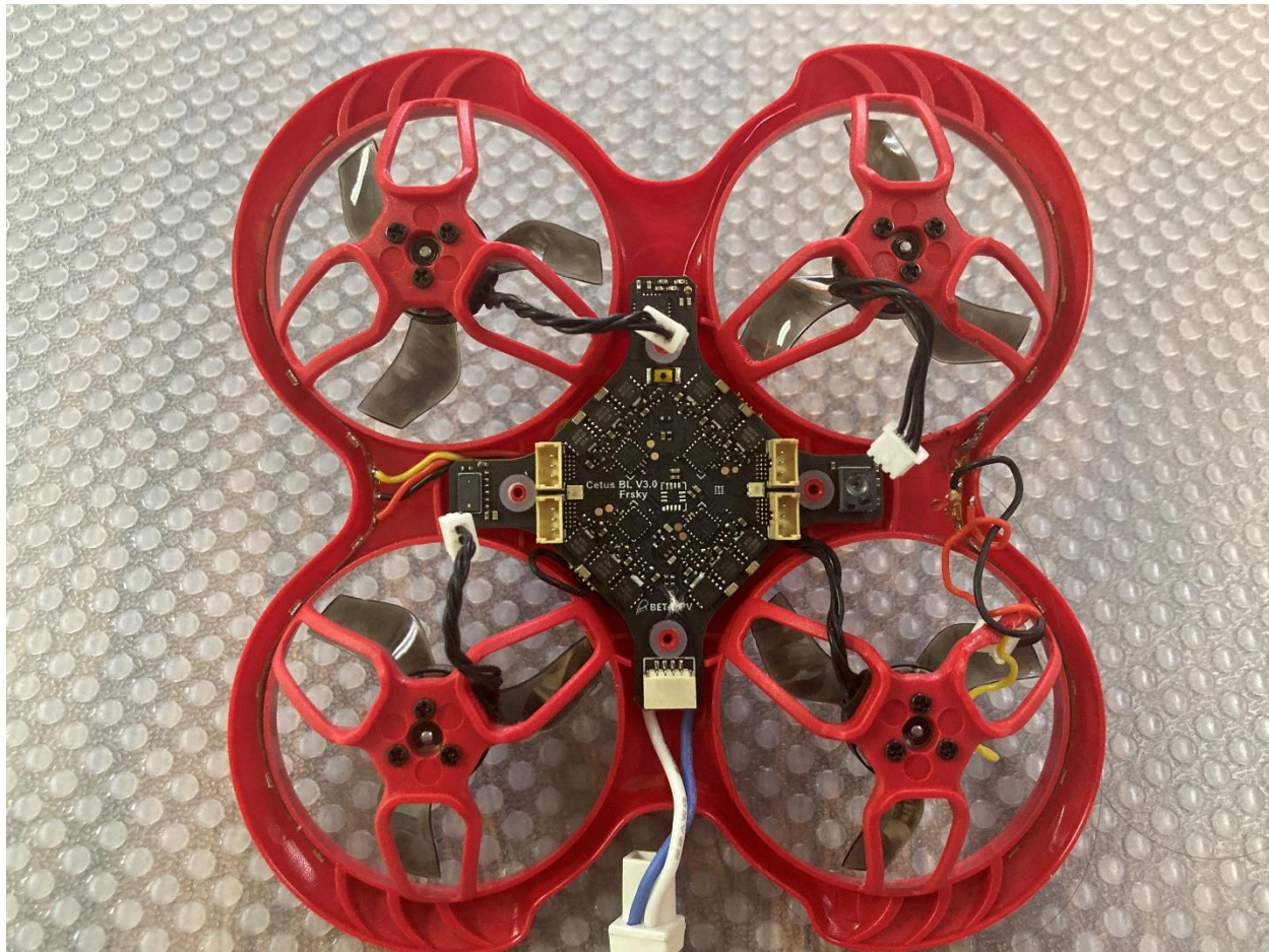
Figure 1. Equipment under Test (cover removed)
