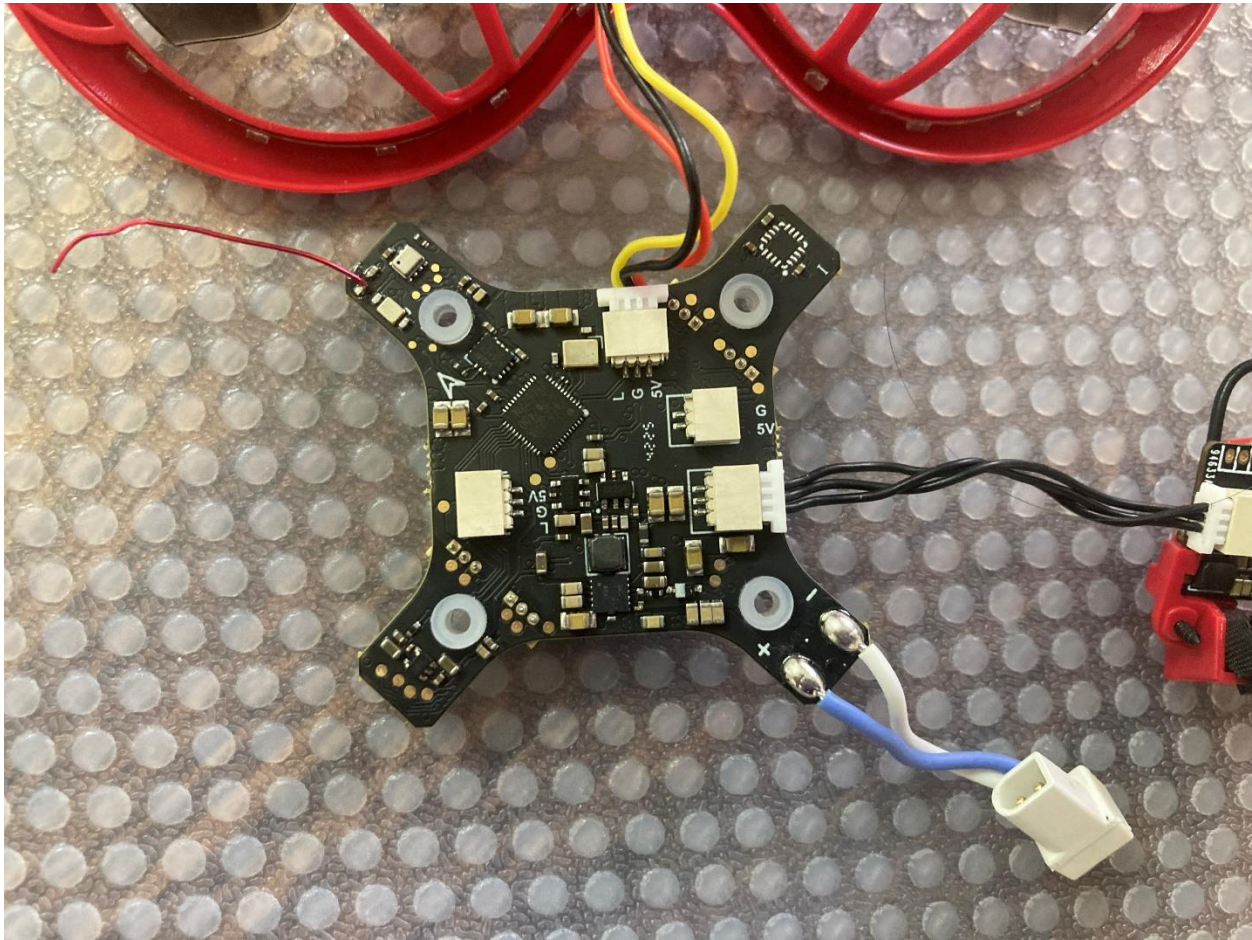
Figure 4. Bottom of primary PCB
