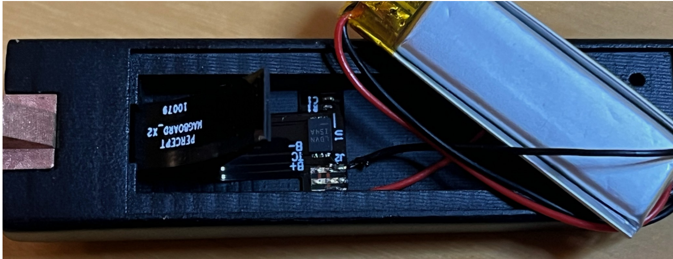
Inside View of the EUT - Battery Side, showing PCB
