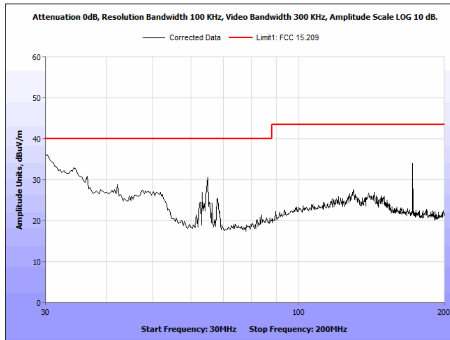
Plot 11. Spurious Emissions Above 30MHz, Out of Band, Horizontal Antenna
