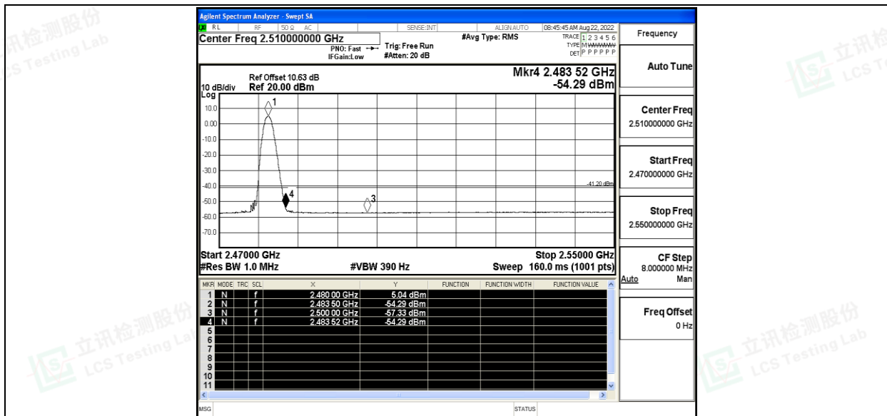
DH5_Ant1_High_2480_Peak
