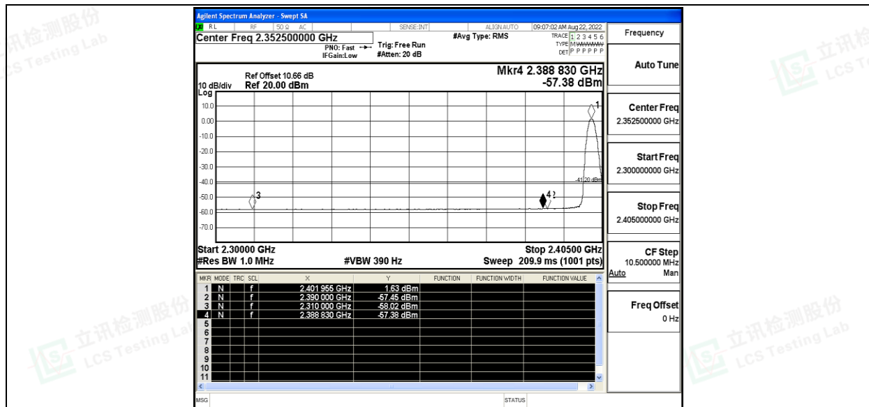
2DH5_Ant1_Low_2402_Peak
