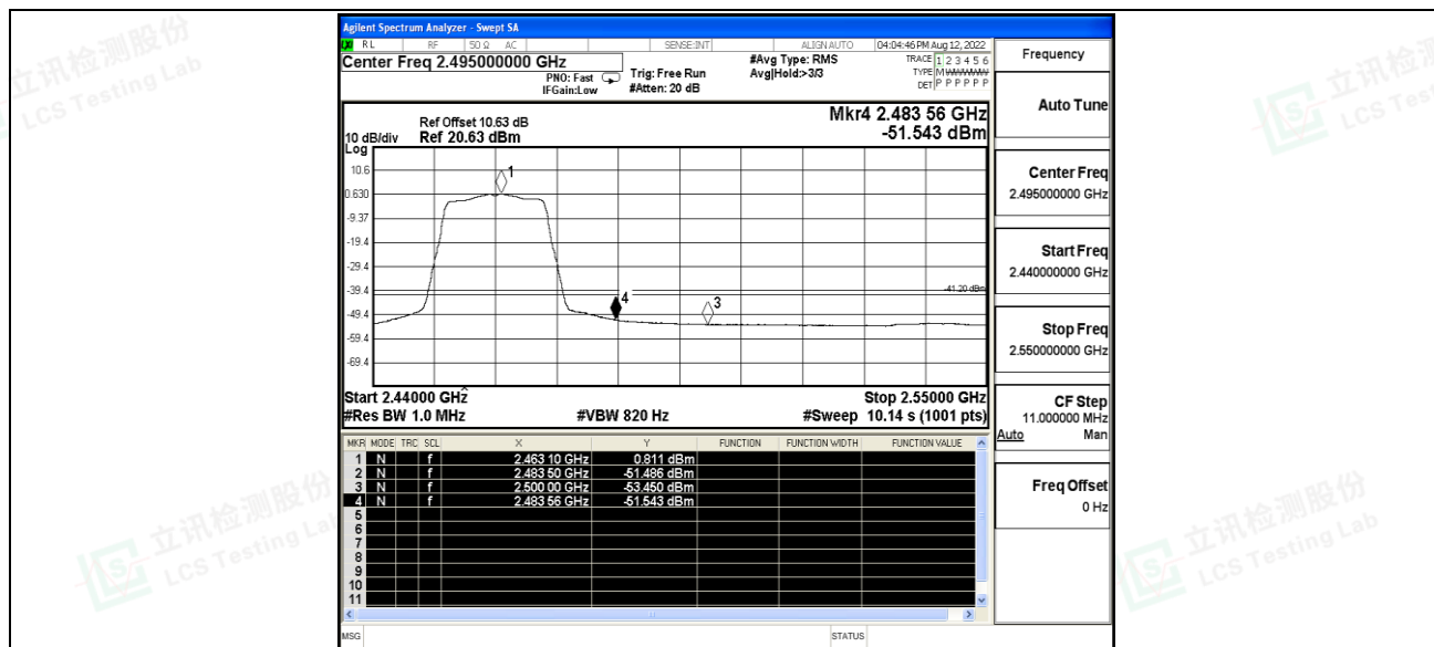
11N20SISO_Ant0_High_2462_Peak
