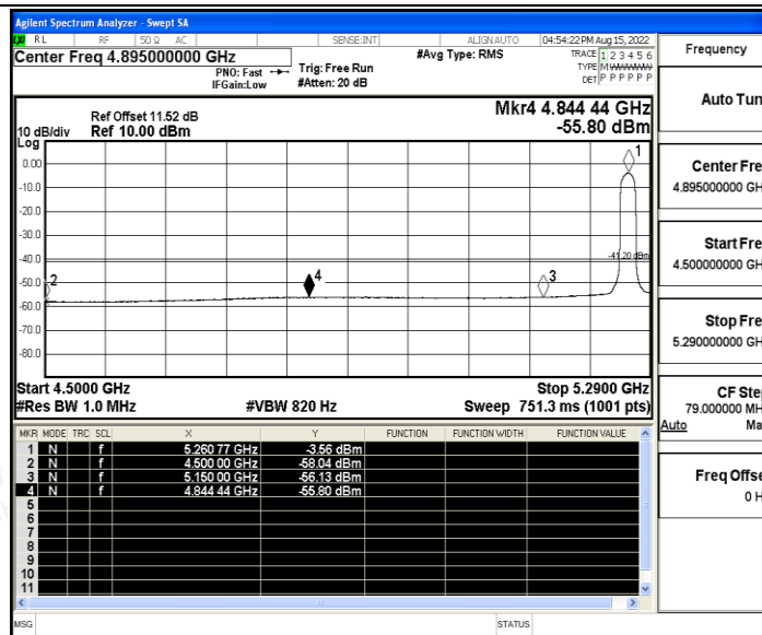
11N20SISO_Ant0_Low_5260_Peak
