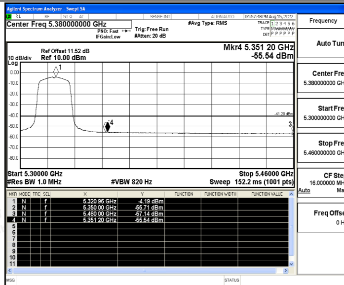
11AC20SISO_Ant0_High_5320_Peak
