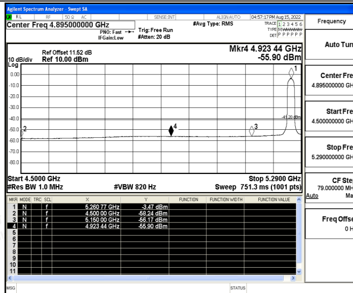
11AC20SISO_Ant0_Low_5260_Peak
