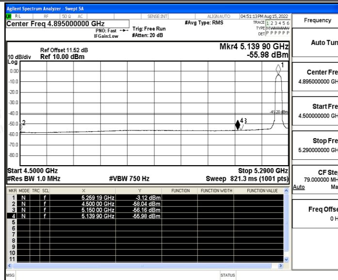
11A_Ant0_Low_5260_Peak
