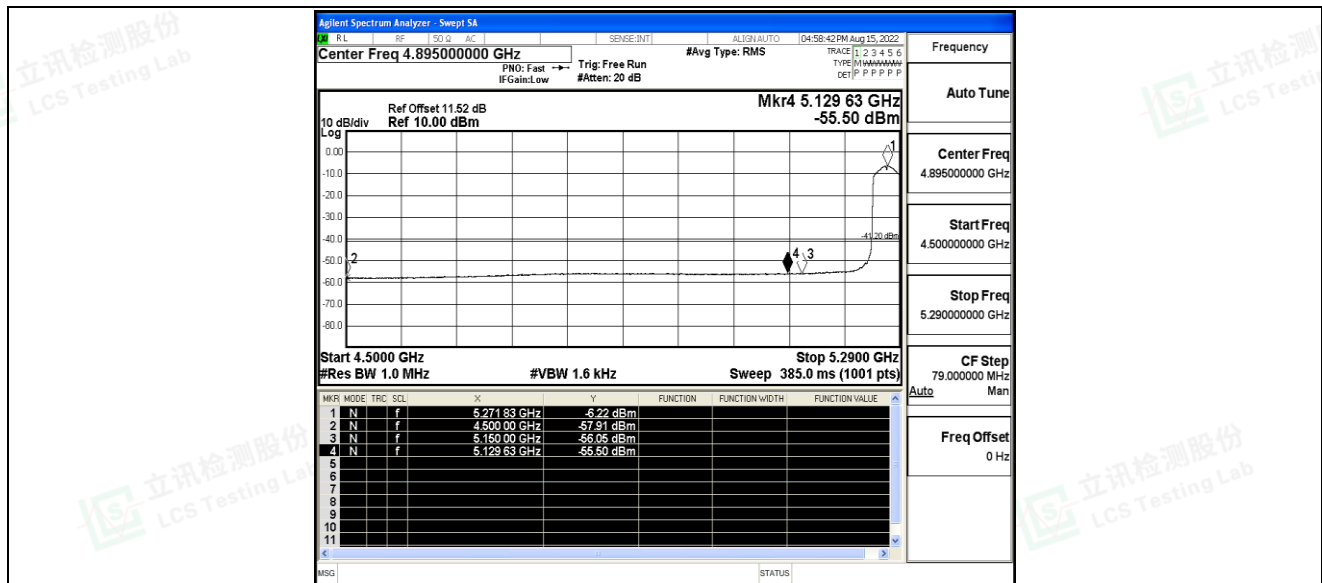
11AC40SISO_Ant0_Low_5270_Peak
