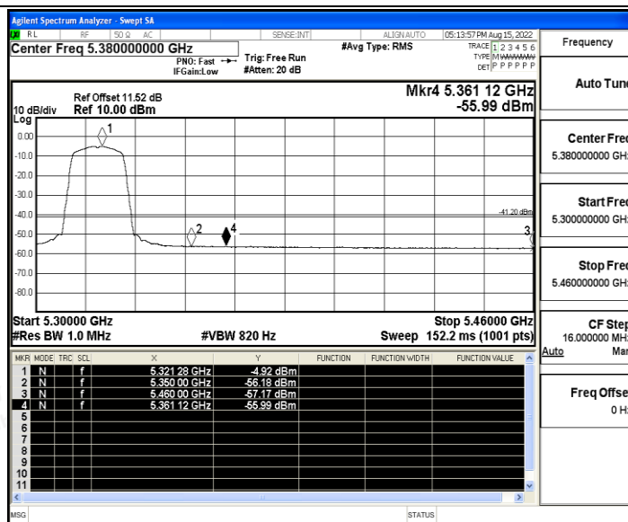
11A_Ant0_High_5320_Peak
