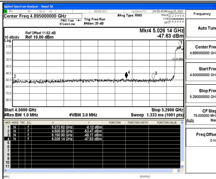
11N40SISO_Ant0_High_5310_AV
