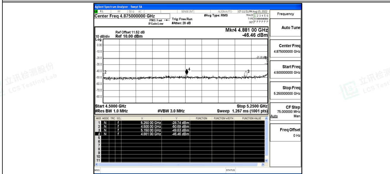
11AC80SISO_Ant1_High_5290_AV
