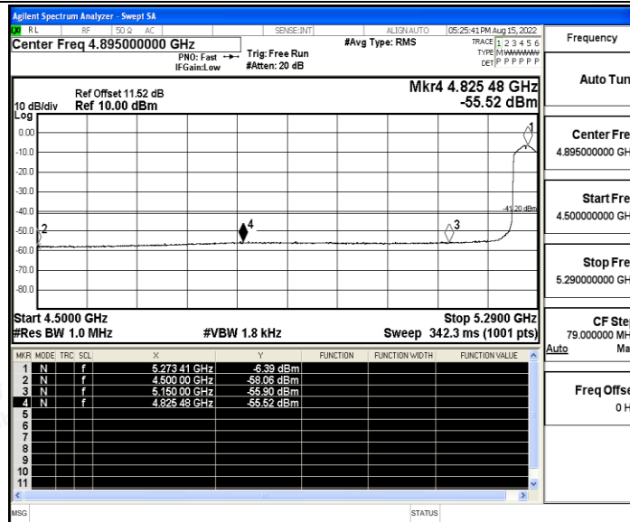
11N40SISO_Ant1_Low_5270_Peak
