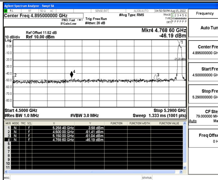
11A_Ant0_High_5320_AV
