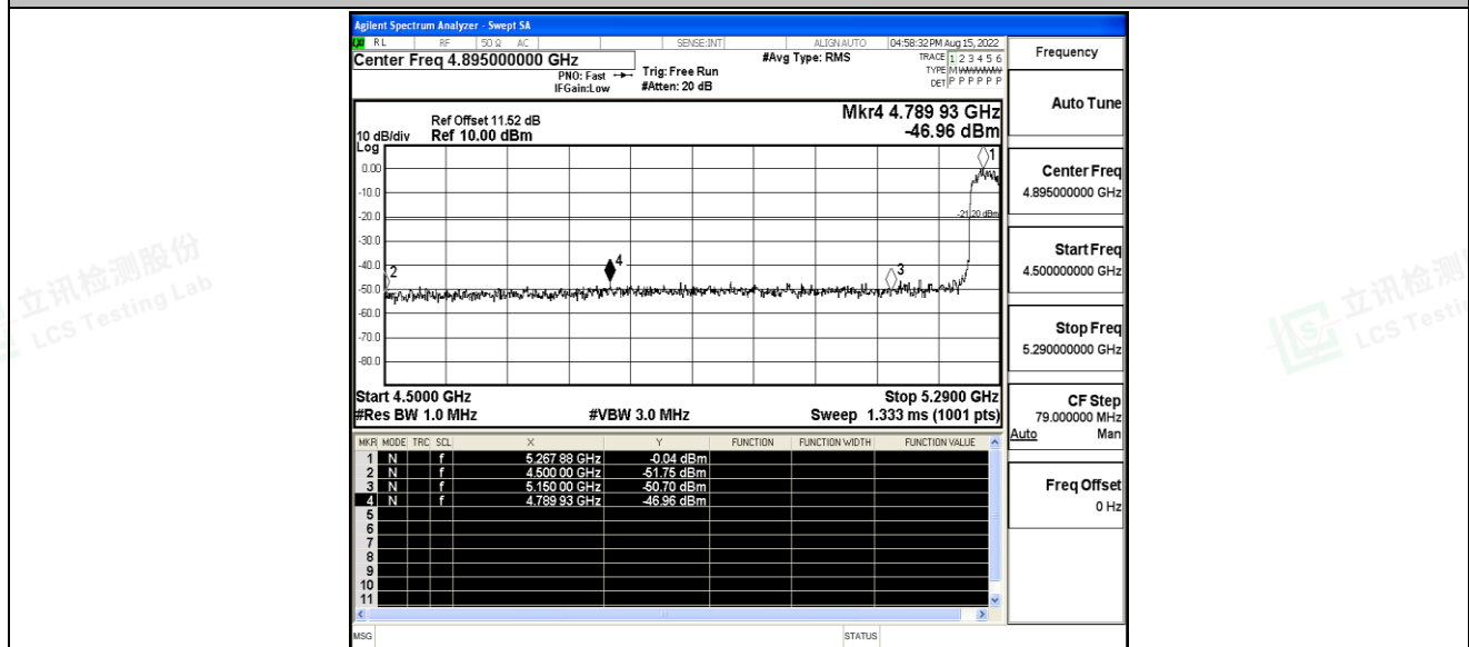
11AC40SISO_Ant0_High_5310_AV
