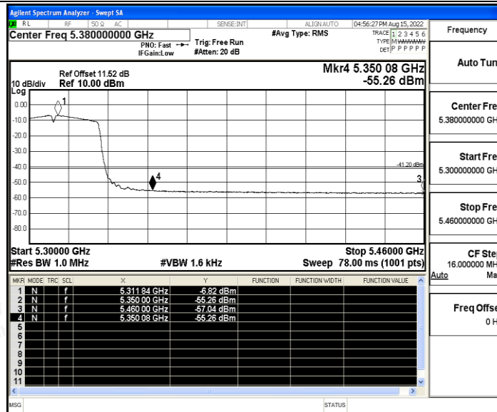
11N40SISO_Ant0_High_5310_Peak
