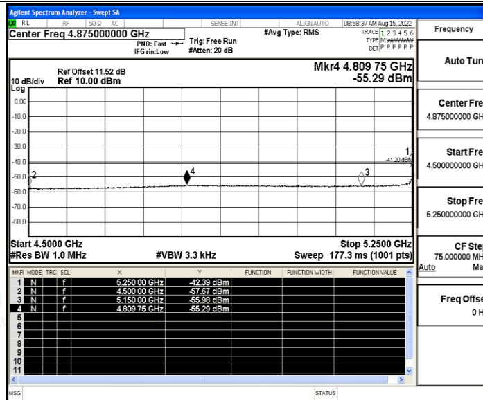
11AC80SISO_Ant0_Low_5290_Peak
