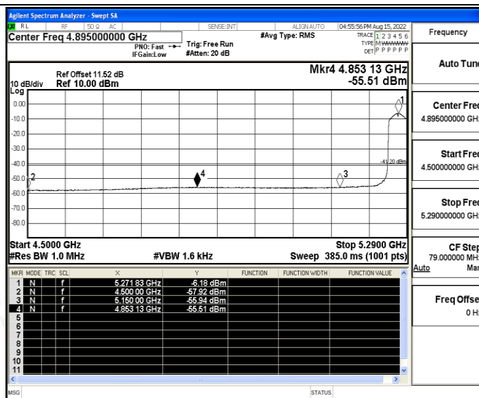
11N40SISO_Ant0_Low_5270_Peak
