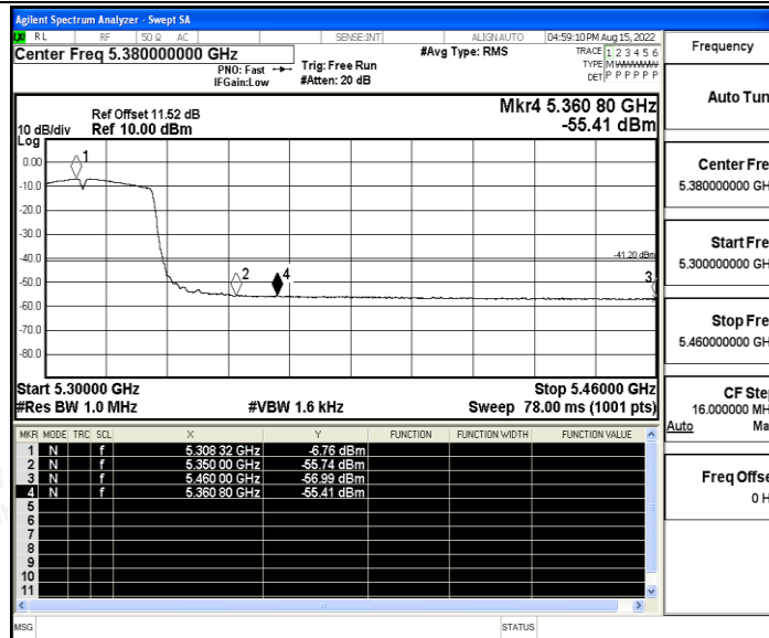
11AC40SISO_Ant0_High_5310_Peak
