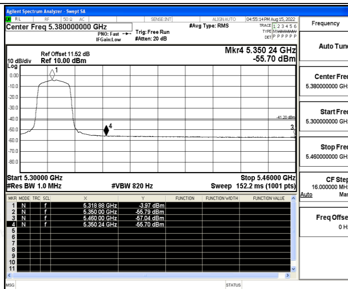
11N20SISO_Ant0_High_5320_Peak
