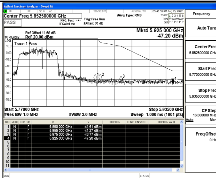
11AC80SISO_Ant0_Low_5775_Peak
