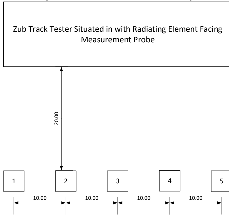
Figure 3 – Test Position 5, Measuring Main Lobe
