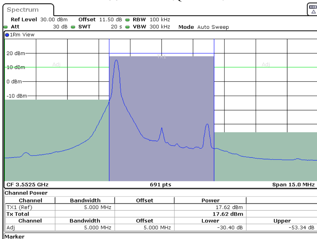
B48-5M-ACLR-L-16QAM-1 RB 0
