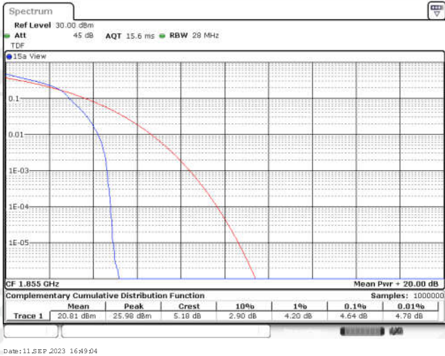
Band25-10MHz-16QAM-26090-50RB#0
