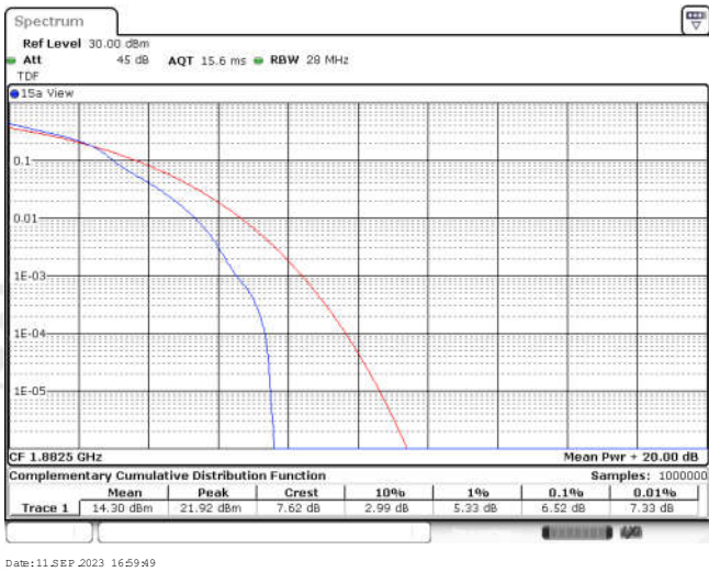
Band25-15MHz-16QAM-26365-75RB#0
