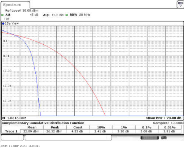
Band25-3MHz-QPSK-26055-15RB#0
