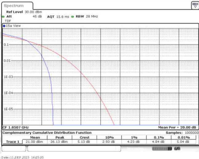
Band25-1.4MHz-16QAM-26047-6RB#0
