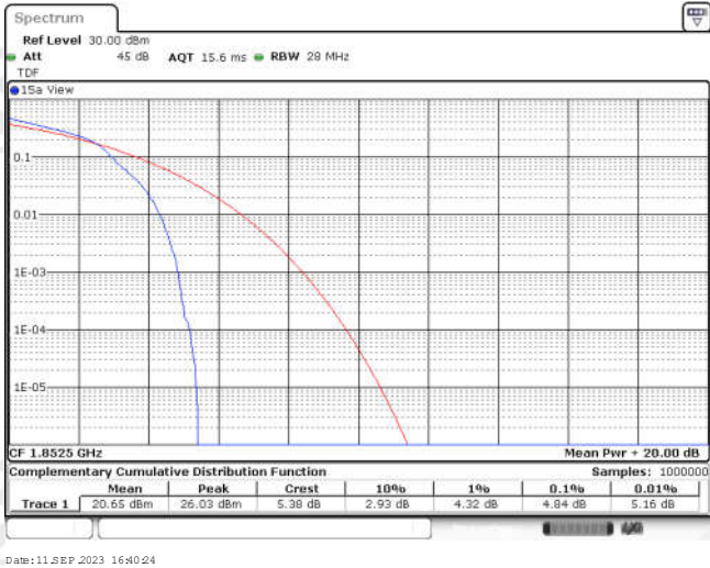
Band25-5MHz-16QAM-26065-25RB#0
