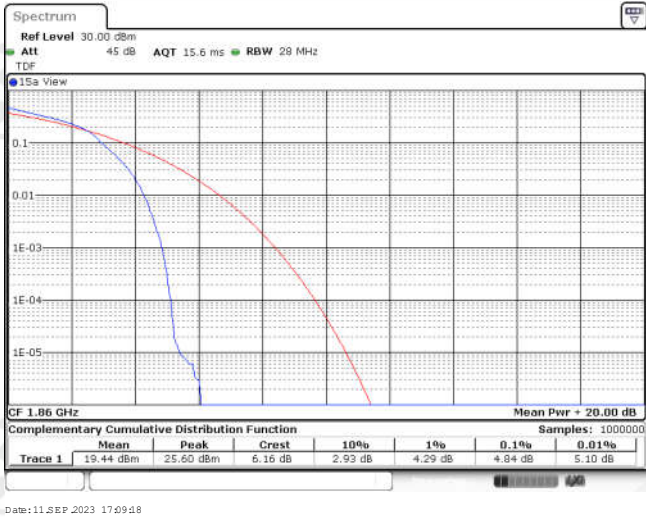
Band25-20MHz-16QAM-26140-100RB#0
