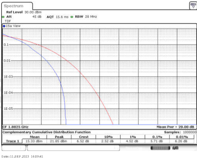
Band25-15MHz-QPSK-26365-75RB#0
