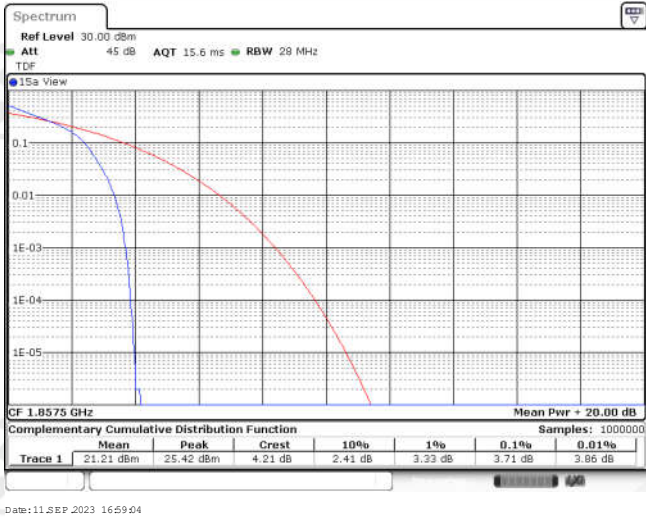
Band25-15MHz-QPSK-26115-75RB#0
