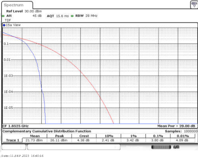
Band25-5MHz-QPSK-26065-25RB#0
