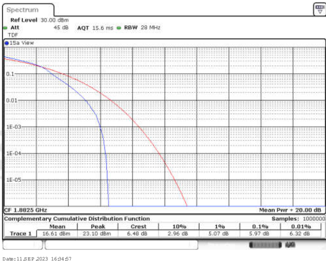
Band25-3MHz-16QAM-26365-15RB#0
