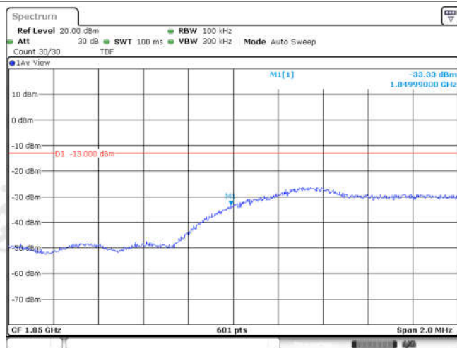
Band25-5MHz-QPSK-26065-25RB#0
