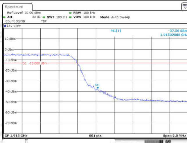
Band25-5MHz-16QAM-26665-25RB#0
