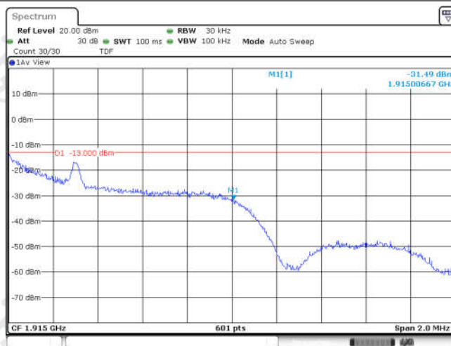
Band25-1.4MHz-QPSK-26683-1RB#0
