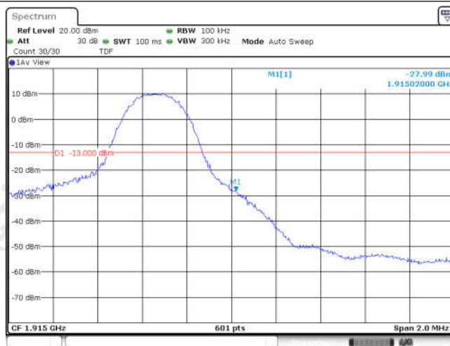
Band25-5MHz-QPSK-26665-25RB#0
