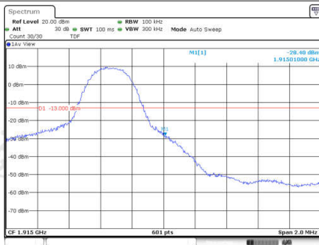
Band25-5MHz-16QAM-26665-25RB#0
