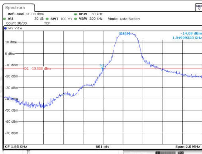
Band25-3MHz-16QAM-26055-1RB#0
