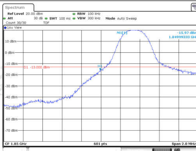
Band25-5MHz-QPSK-26065-1RB#0
