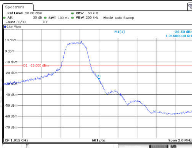
Band25-3MHz-16QAM-26675-15RB#0
