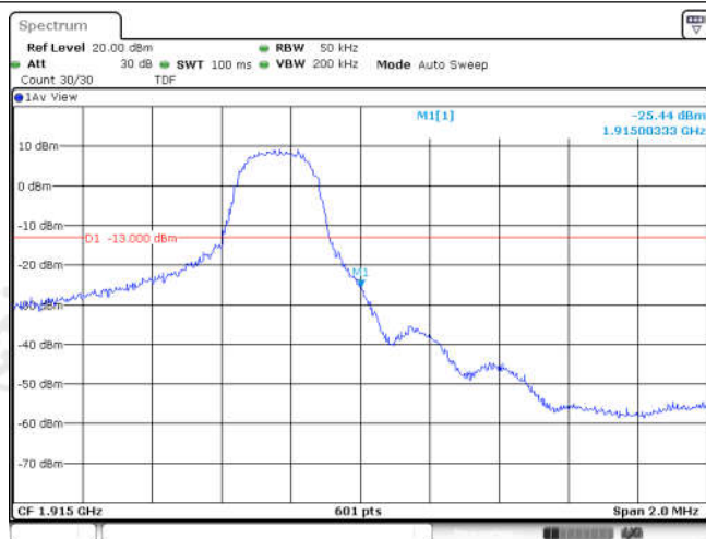
Band25-3MHz-QPSK-26675-15RB#0
