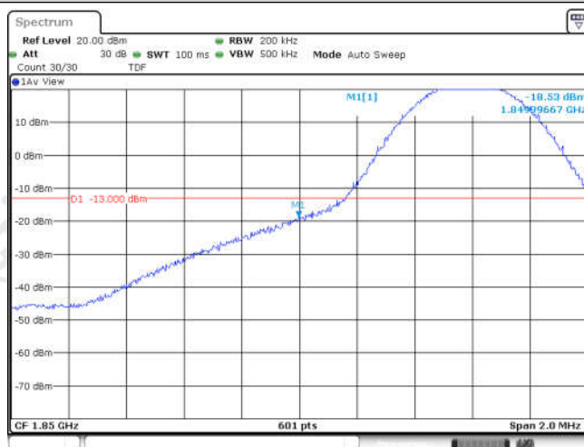
Band25-10MHz-QPSK-26090-1RB#0
