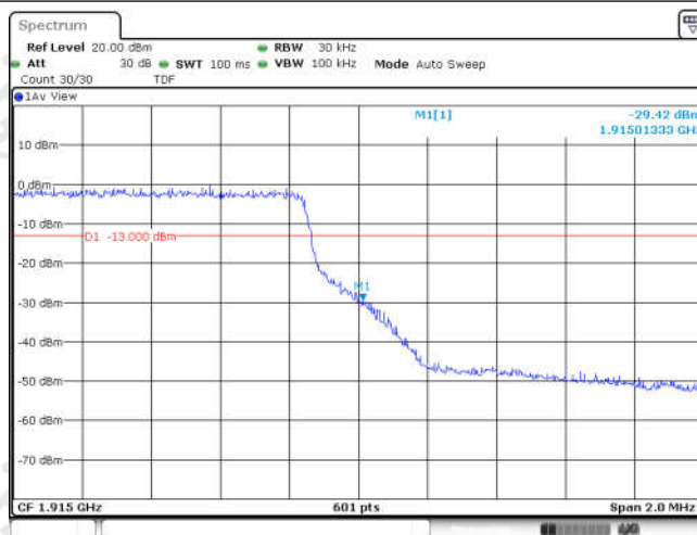
Band25-1.4MHz-16QAM-26683-6RB#0
