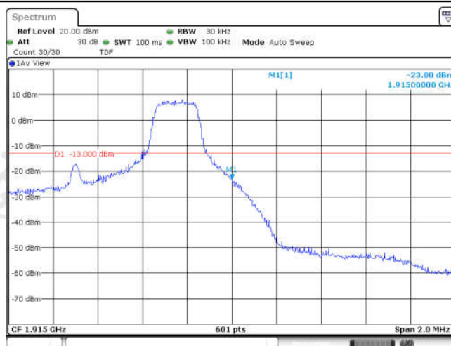
Band25-1.4MHz-QPSK-26683-1RB#5
