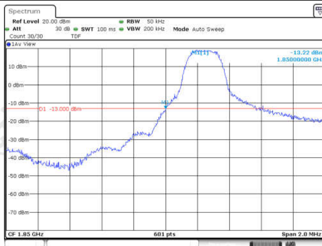
Band25-3MHz-QPSK-26055-1RB#0
