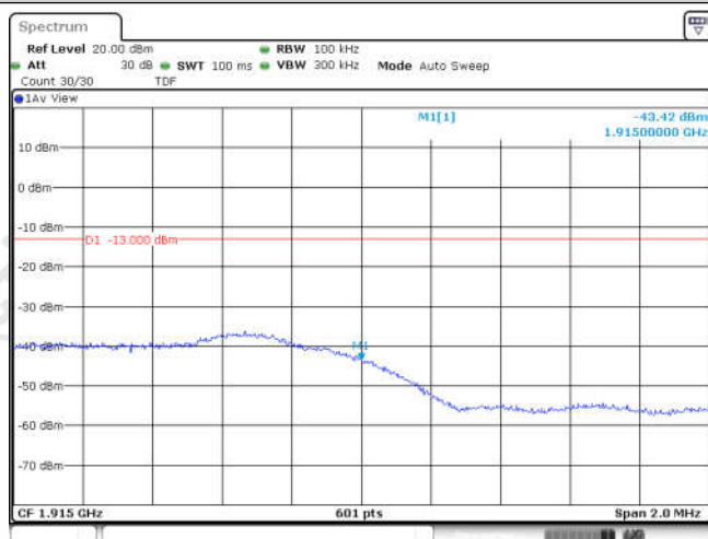
Band25-5MHz-QPSK-26665-1RB#0
