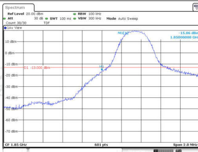
Band25-5MHz-16QAM-26065-1RB#0
