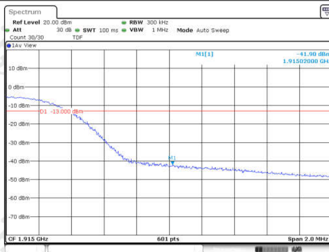
Band25-15MHz-16QAM-26615-75RB#0
