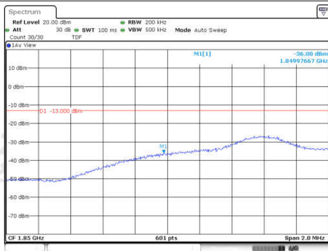
Band25-10MHz-16QAM-26090-50RB#0
