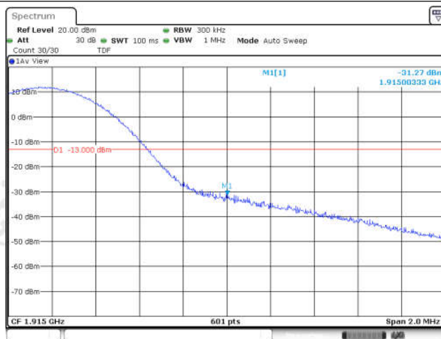
Band25-15MHz-16QAM-26615-75RB#0
