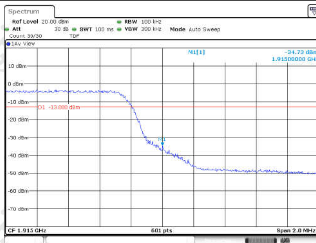
Band25-5MHz-QPSK-26665-25RB#0
