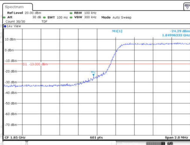
Band25-5MHz-QPSK-26065-25RB#0
