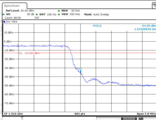
Band25-3MHz-16QAM-26675-15RB#0
