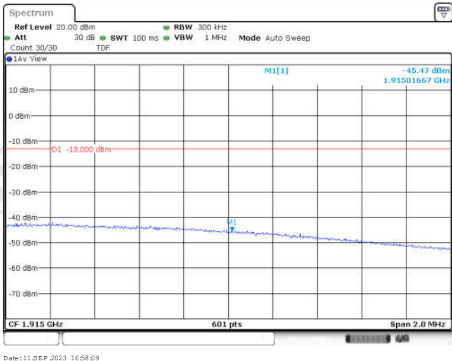
Band25-15MHz-16QAM-26615-1RB#74
