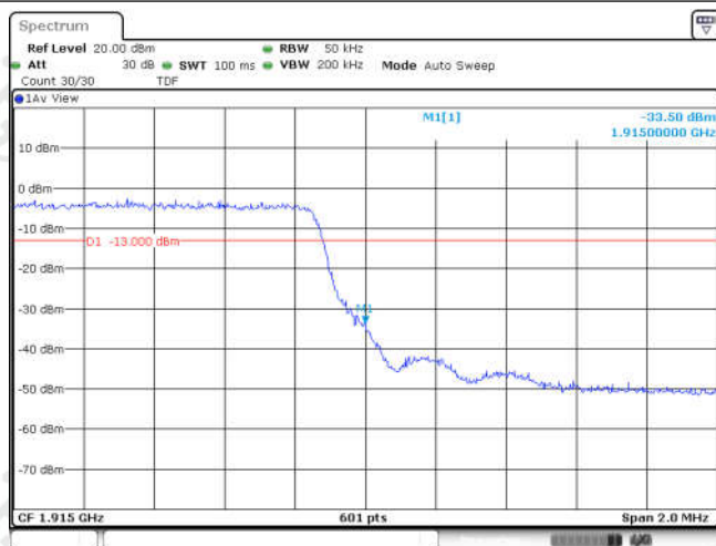
Band25-3MHz-QPSK-26675-15RB#0
