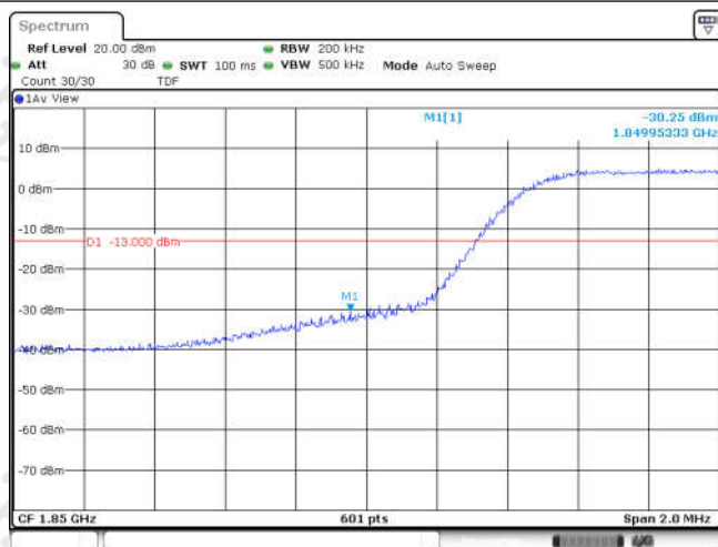
Band25-10MHz-16QAM-26090-50RB#0
