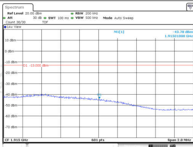
Band25-10MHz-16QAM-26640-1RB#0
